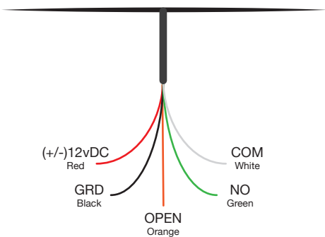
Cable Diagram
