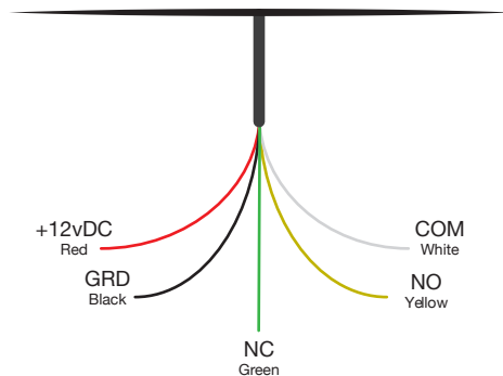
Cable Diagram
