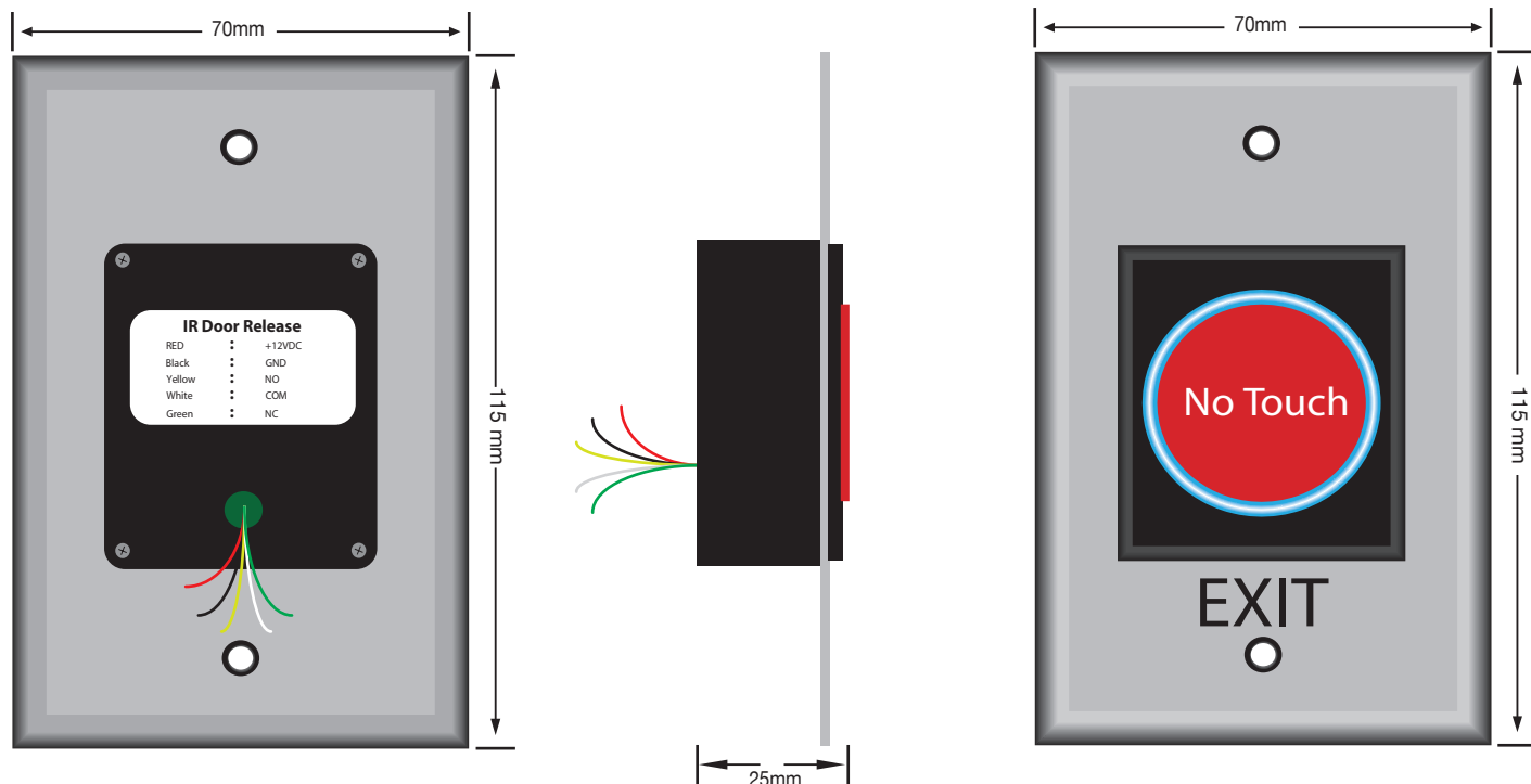
Cable Diagram
