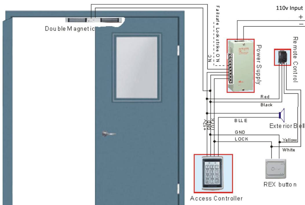
Access Control Installation Diagram for Magnetic lock for double doors
