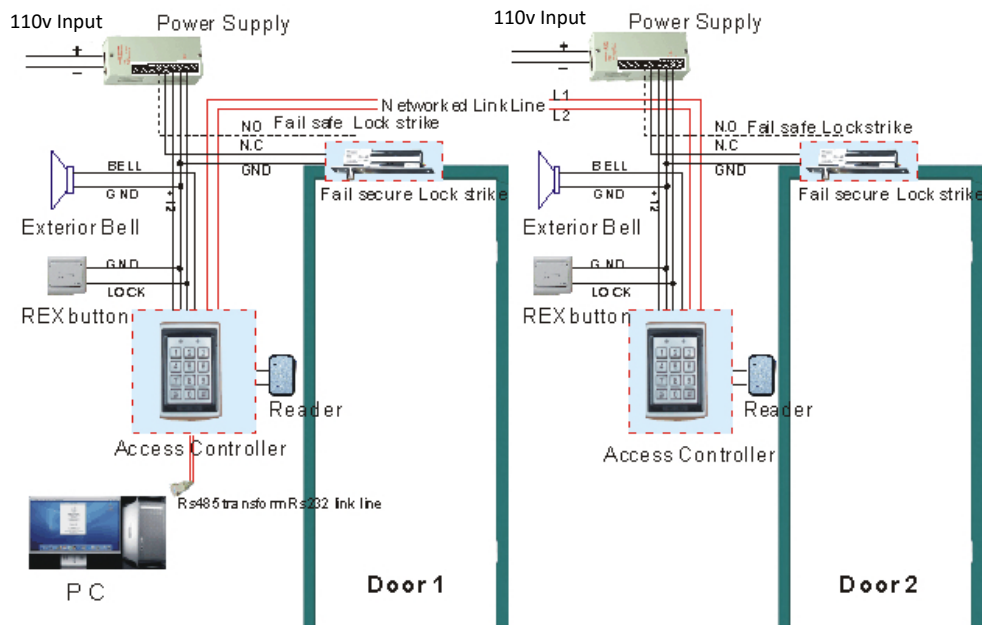
Installation Diagram for Multi Networked doors
