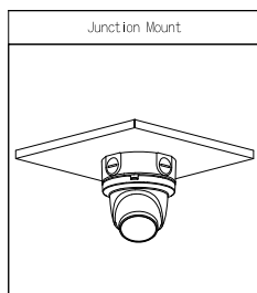
JBEW-130 Water-proof Junction Box
