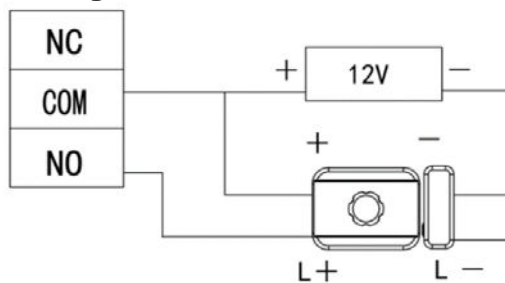
Figure 2-6 Electric lock
