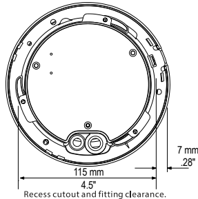
Recess cutout and fitting clearance.
