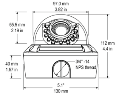
Camera Dimensions
