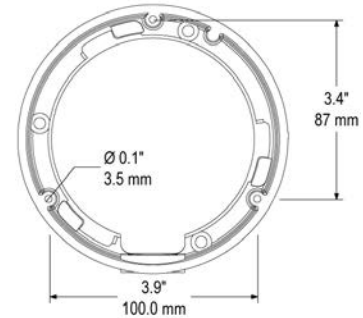
Base Hole Screw Dimensions
