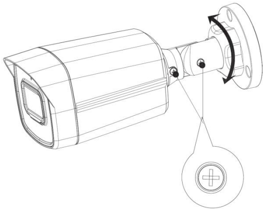
Figure 3-2-27 Model L adjustment
