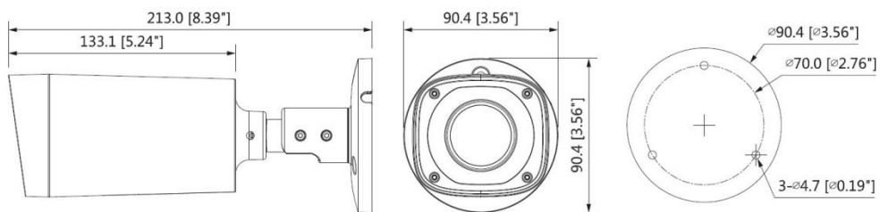
Figure 2-2-2 Model A (2) (mm [in.])
