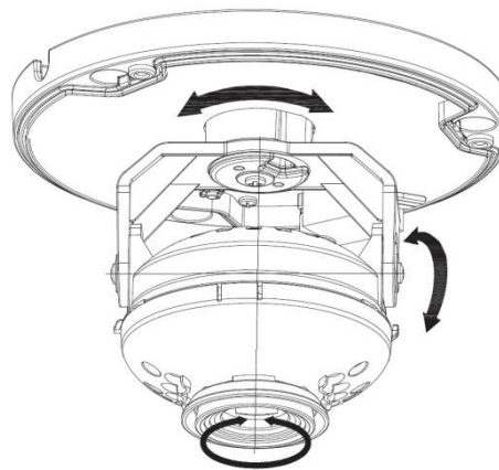
Figure 3-3-2 Model A adjustment
