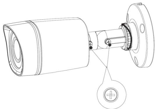
Figure 3-2-15 Model G adjustment
