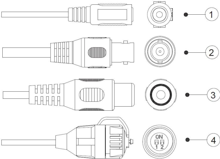
Figure 2-8 Cable list
