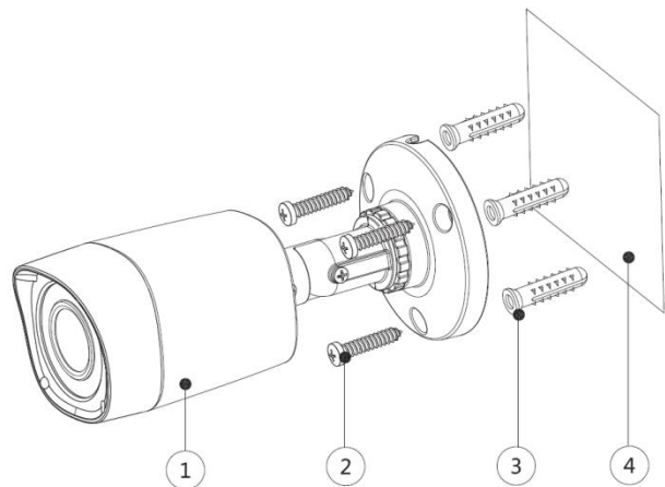
Figure 3-2-14 Model G installation
