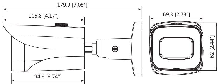
Figure 2-1 Model A (mm [in])
