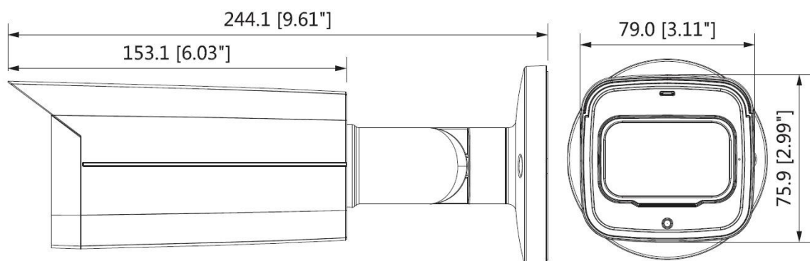
Figure 2-4 Model D (mm [in]) and Model E (mm [in])
