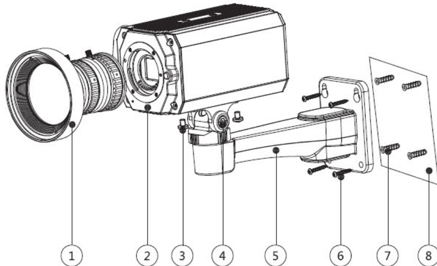
Figure 9-6 Device components
