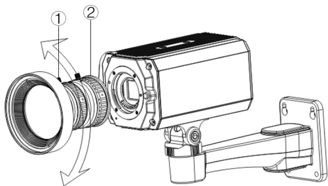
Figure 9-3 Lens installation (2)
