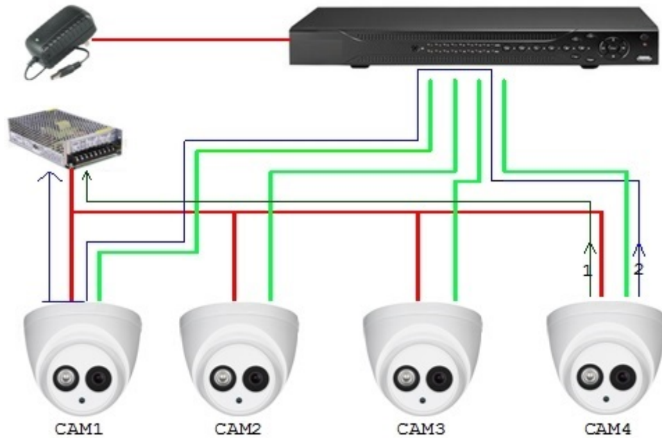
Figure 11-1 Principle of centralized power supply
