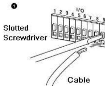
Figure 9-4 Install cable
