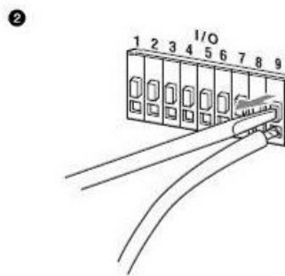
Figure 9-5 Remove cable
