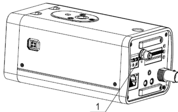
Figure 3-10 3G/Wifi antenna installation 1
