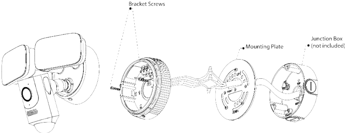
Figure 2-1 Assembly
