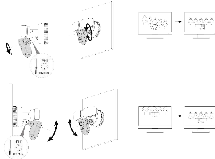
Figure 6-3 Adjust the lens angle (1)
