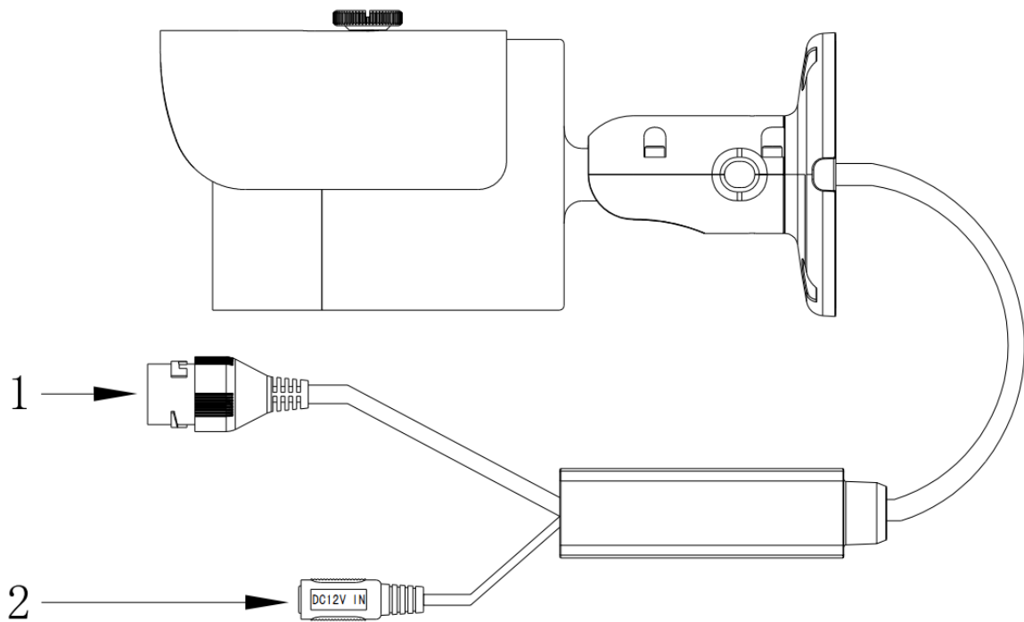
Figure 2-1 Cable
