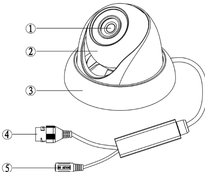
Figure 2-2 Plastic Dome
