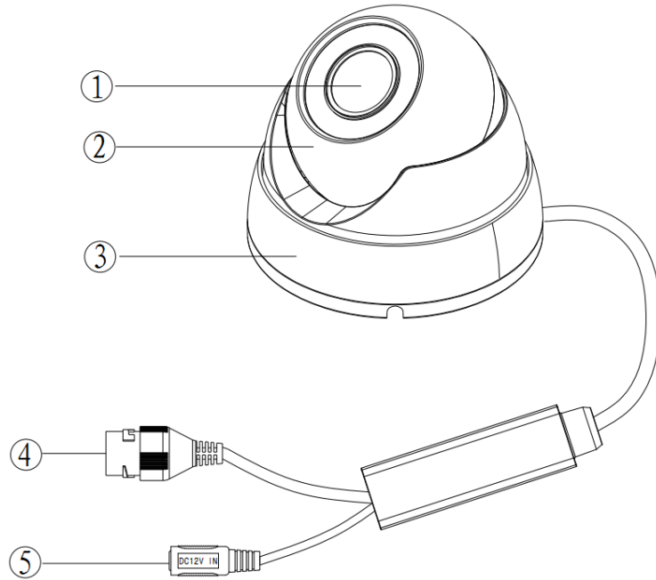
Figure 2-1 Metal Dome
