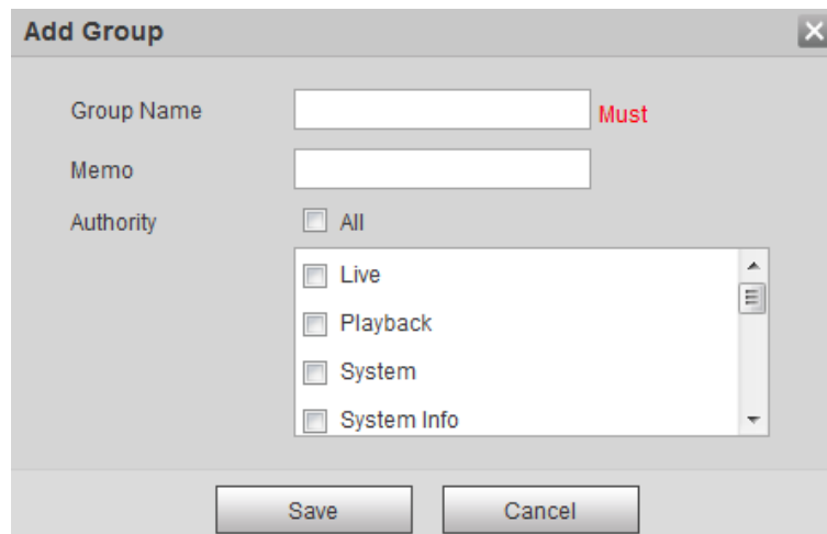
Figure 4-87 Add Group
