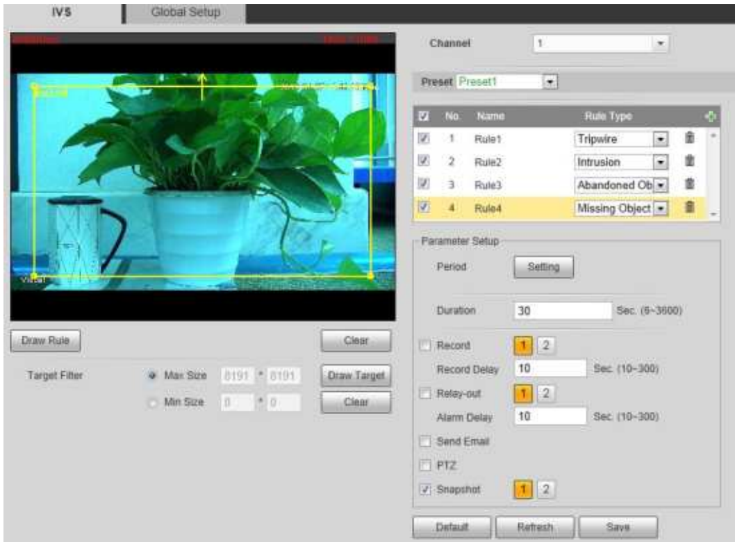
Figure 4-46 Missing object
