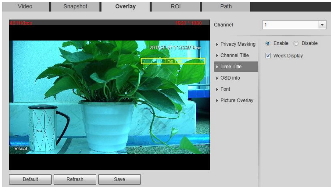
Figure 4-17 Time title
