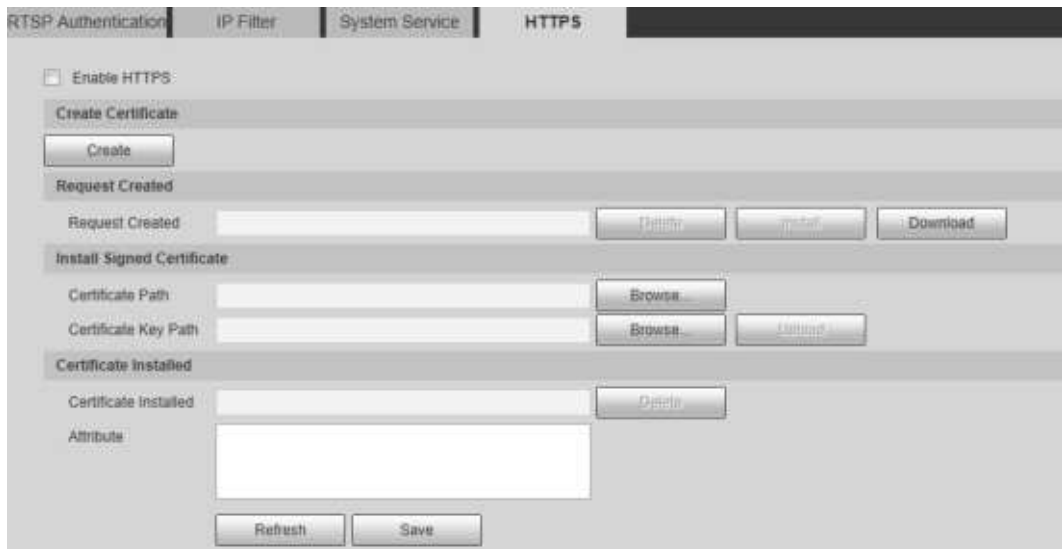
Figure 4-107 HTTPS
