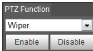
Figure 3-11 Wiper
