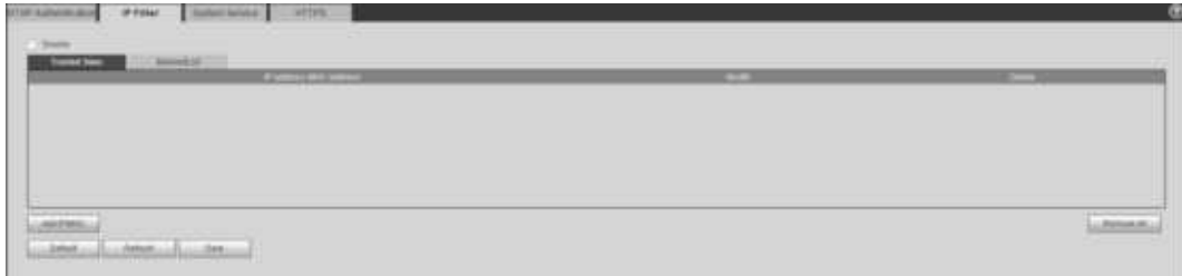
Figure 4-97 IP filter
