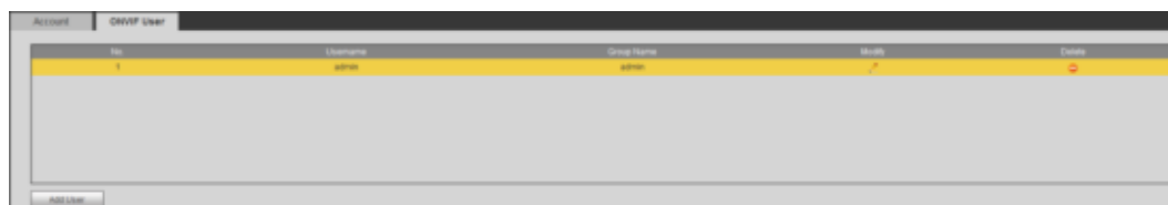
Figure 4-94 ONVIF user
