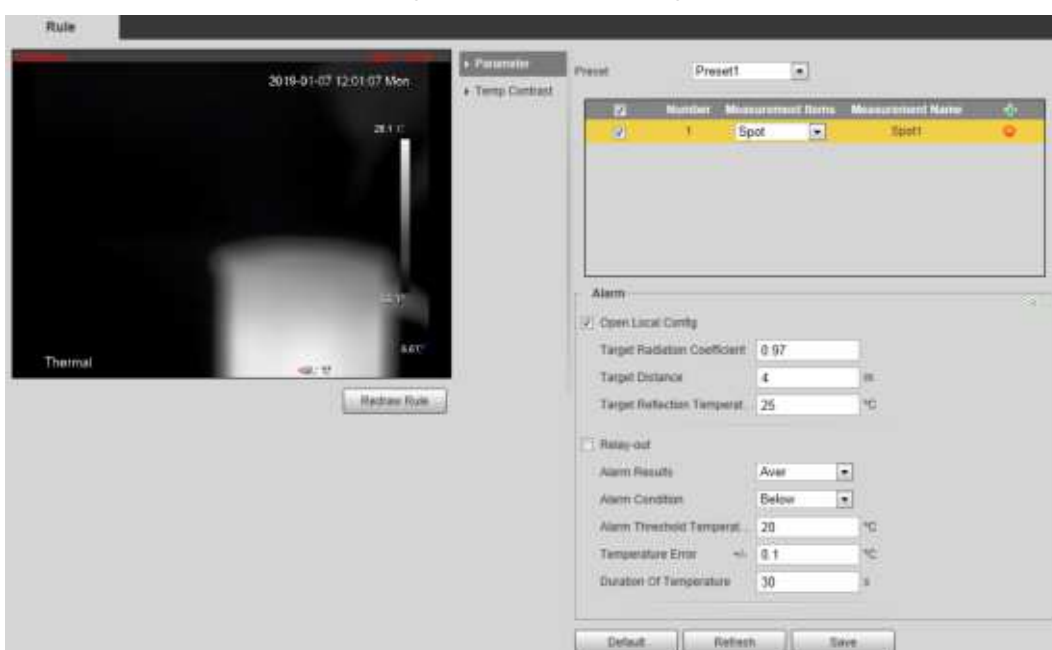
Figure 4-65 Rule adding
