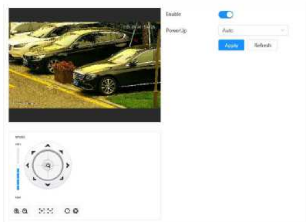
Figure 4-60 PowerUp
