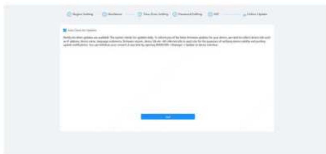
Figure 3-6 Online update
