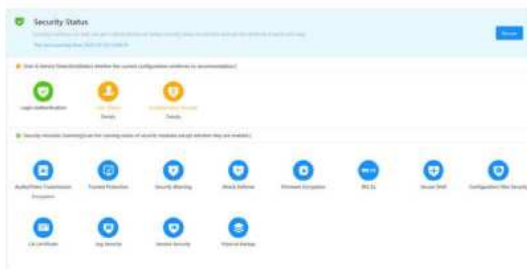
Figure 10-1 Security status
