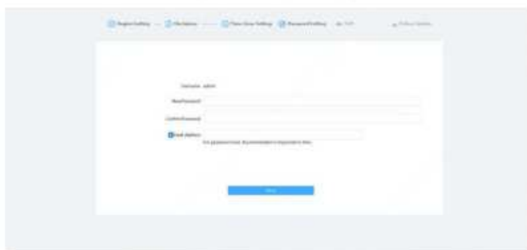
Figure 3-4 Password setting
