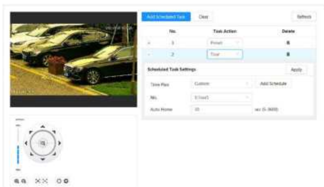
Figure 4-62 Scheduled task
