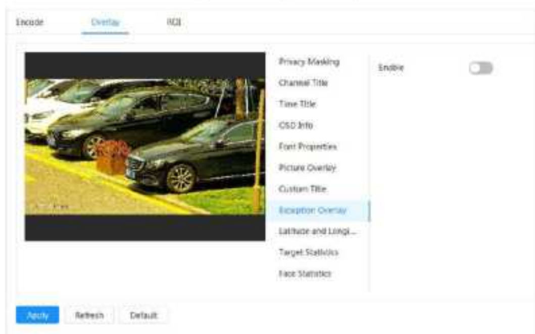
Figure 4-25 Exception overlay
