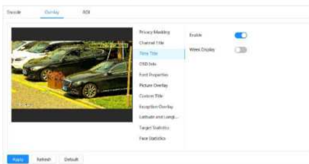
Figure 4-20 Time title
