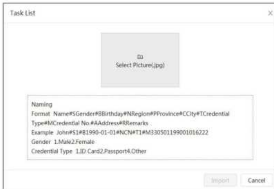
Figure 9-14 Task list
