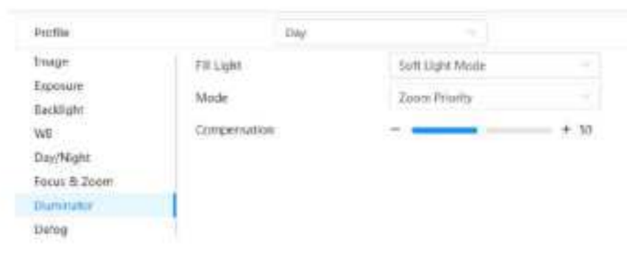
Figure 4-14 Illuminator (2)
