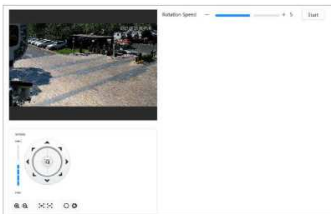
Figure 4-57 Pan
