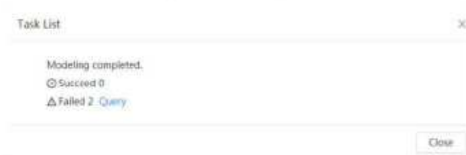
Figure 9-16 Modeling result
