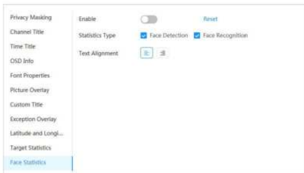
Figure 4-28 Face statistics
