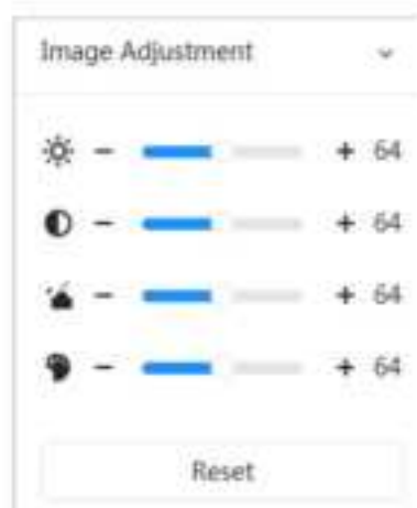
Figure 6-8 Image adjustment
