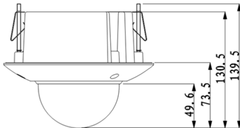
Figure 2-2 Dimension 2
