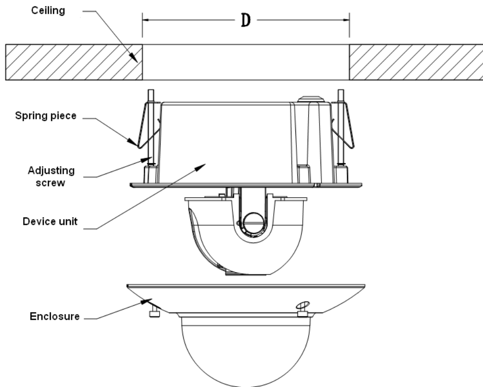
Figure 3-1 Installation diagram
