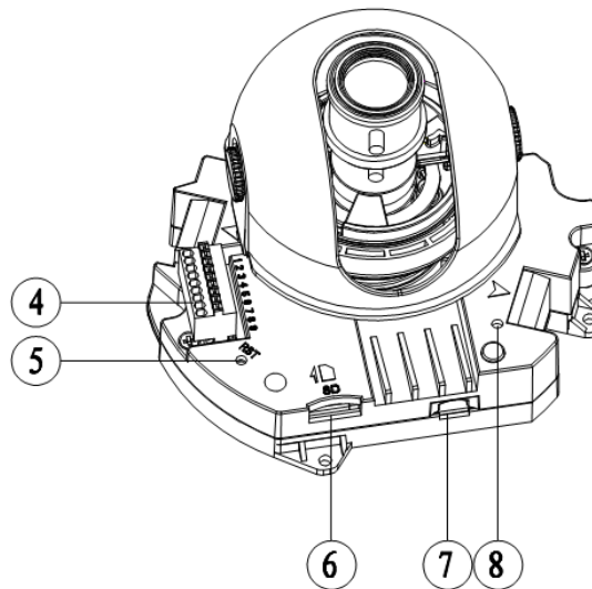
Figure 2-4 Port 2
