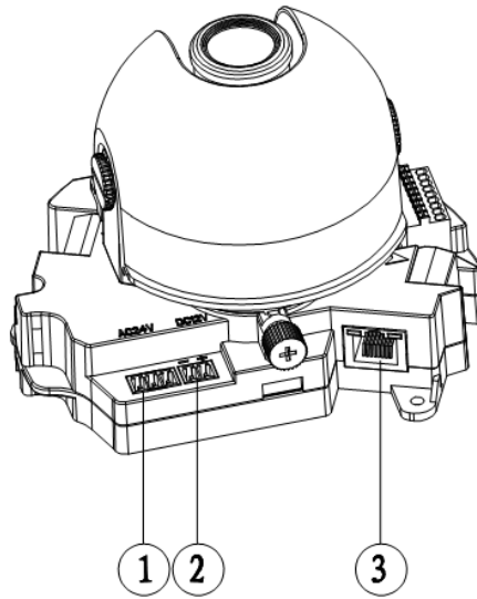
Figure 2-3 Port 1
