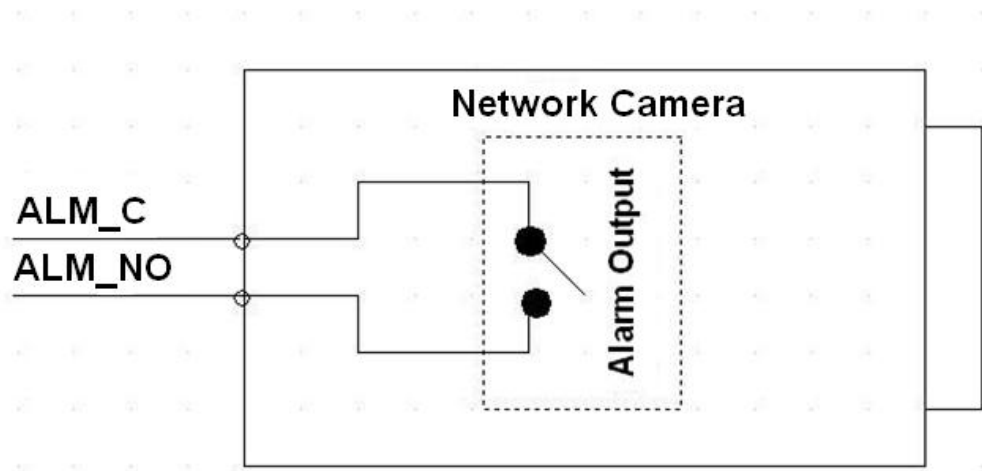
Figure 2-14 Alarm output
