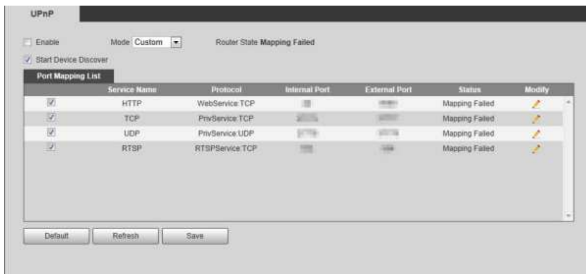
Figure 4-81 UPnP
