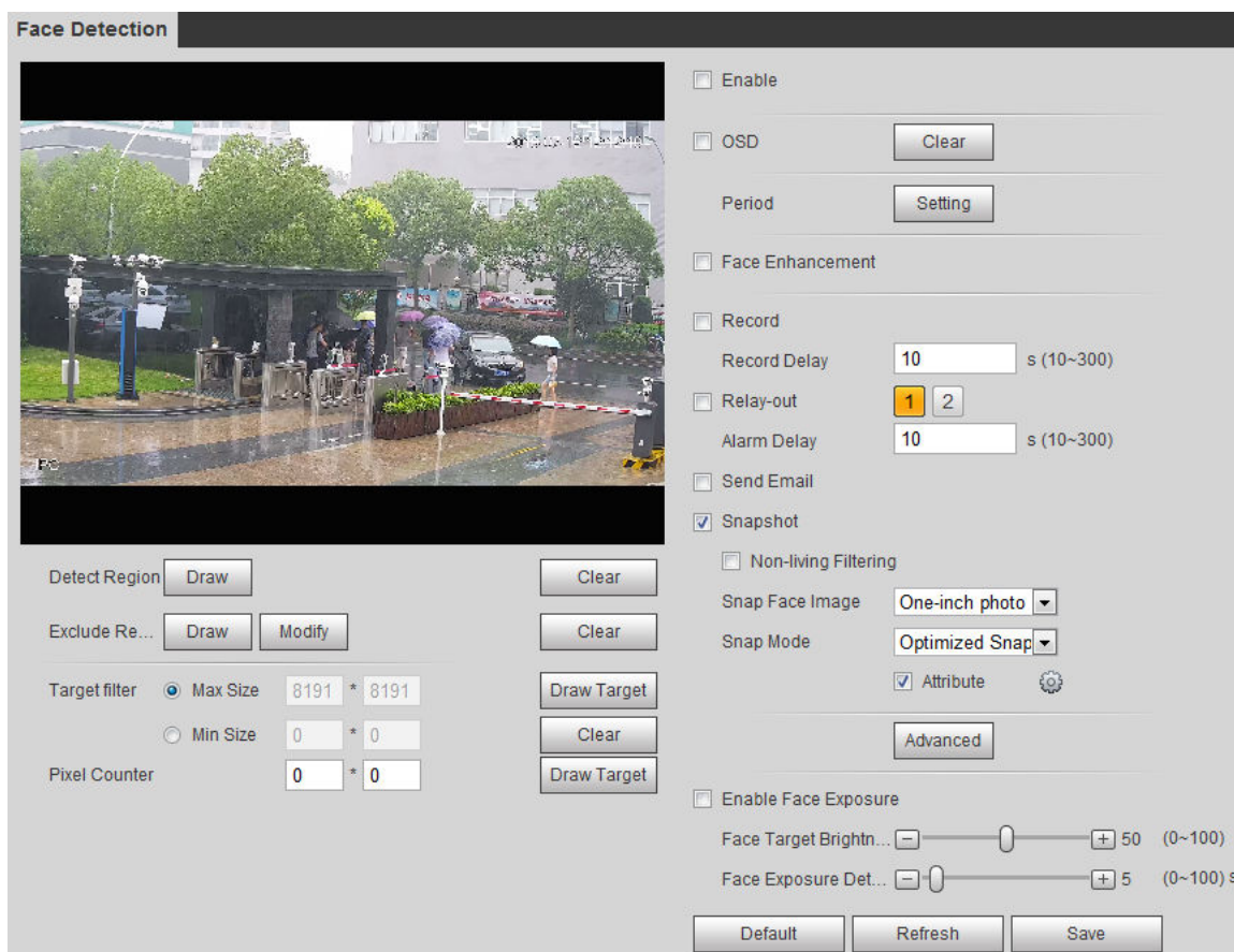
Figure 5-62 Face detection
