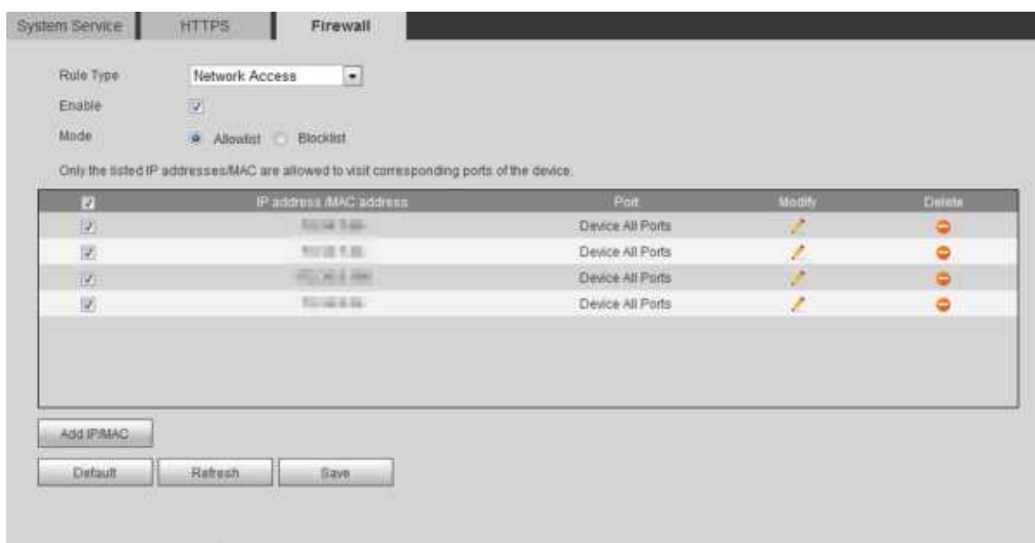
Figure 4-123 Firewall
