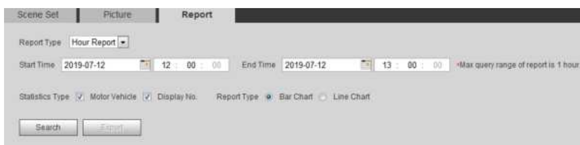
Figure 5-86 Report
