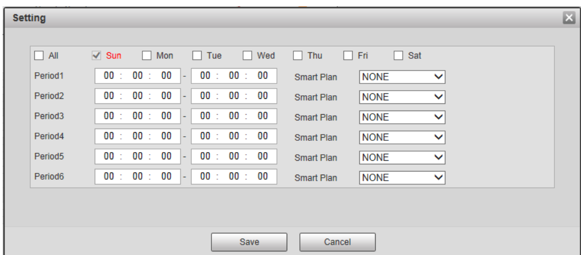
Figure 5-31 Time settings (1)
