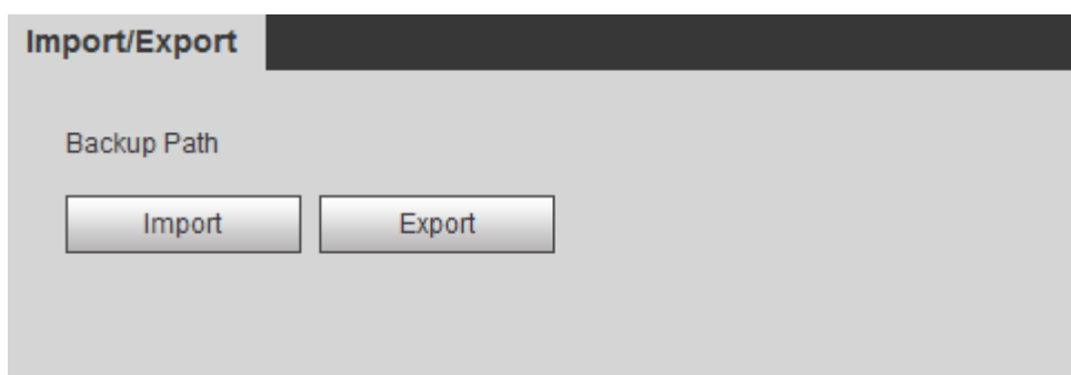
Figure 6-6 Import/Export
