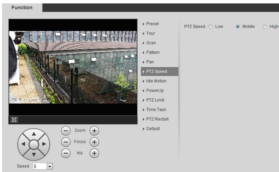
Figure 4-13 PTZ speed
