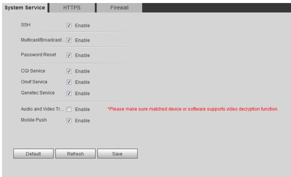
Figure 4-113 System service
