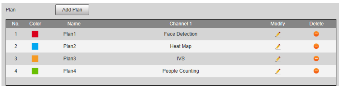
Figure 5-30 Add plan (2)
