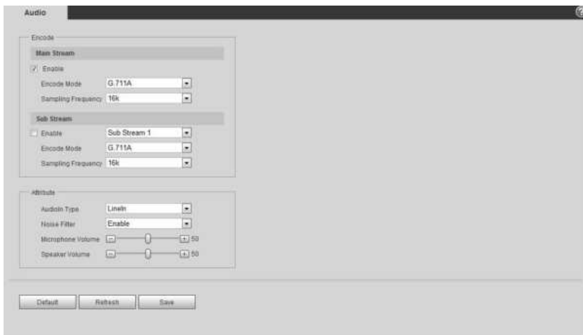
Figure 4-73 Audio
