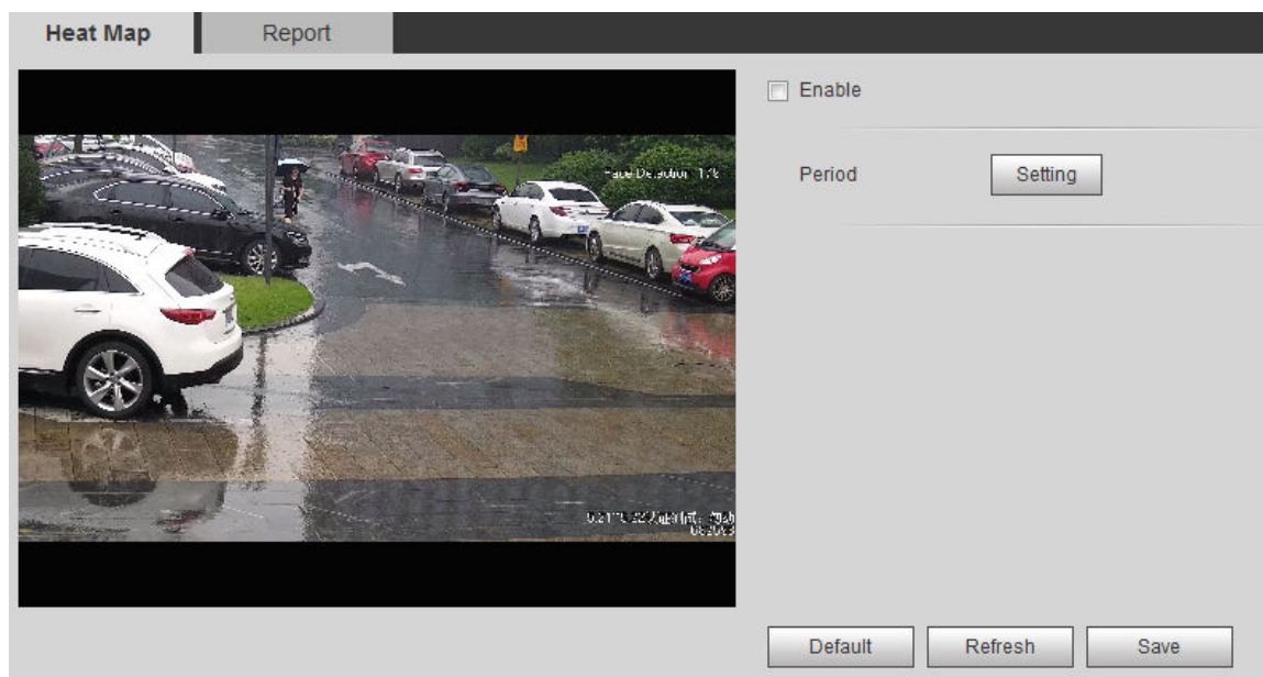
Figure 5-73 Heat map
