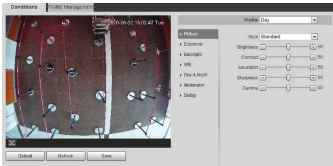
Figure 4-32 Camera conditions
