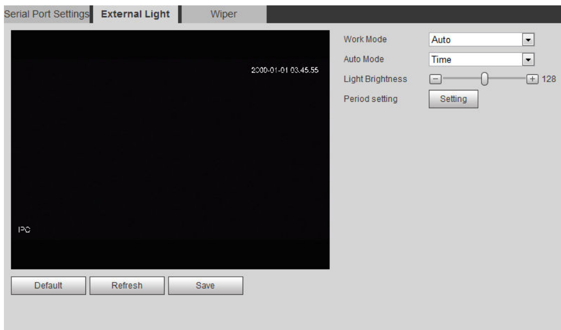
Figure 4-126 External light
