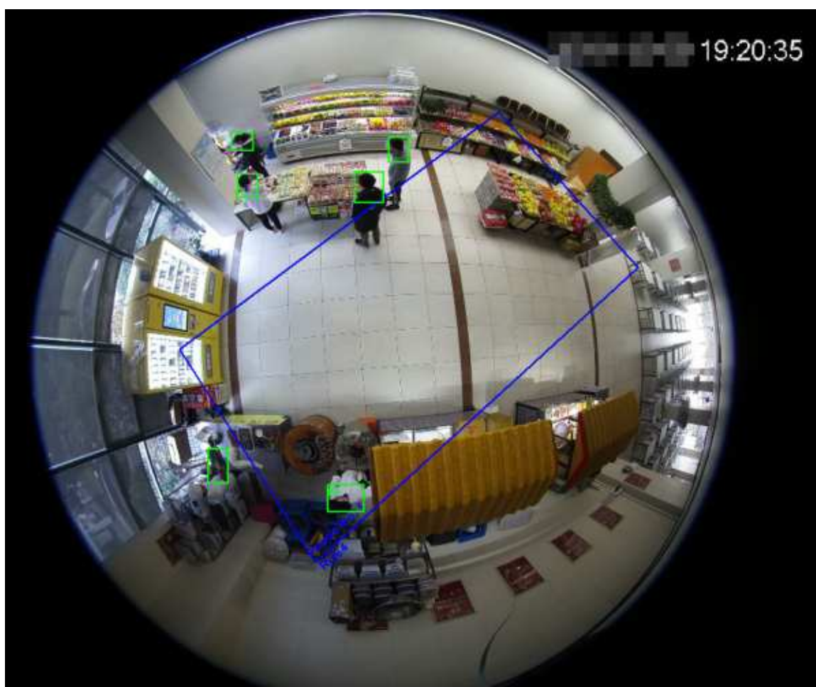
Figure 5-69 Queuing result
