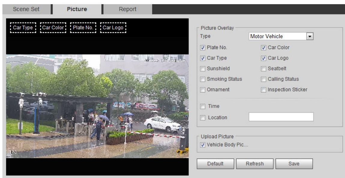
Figure 5-85 Picture
