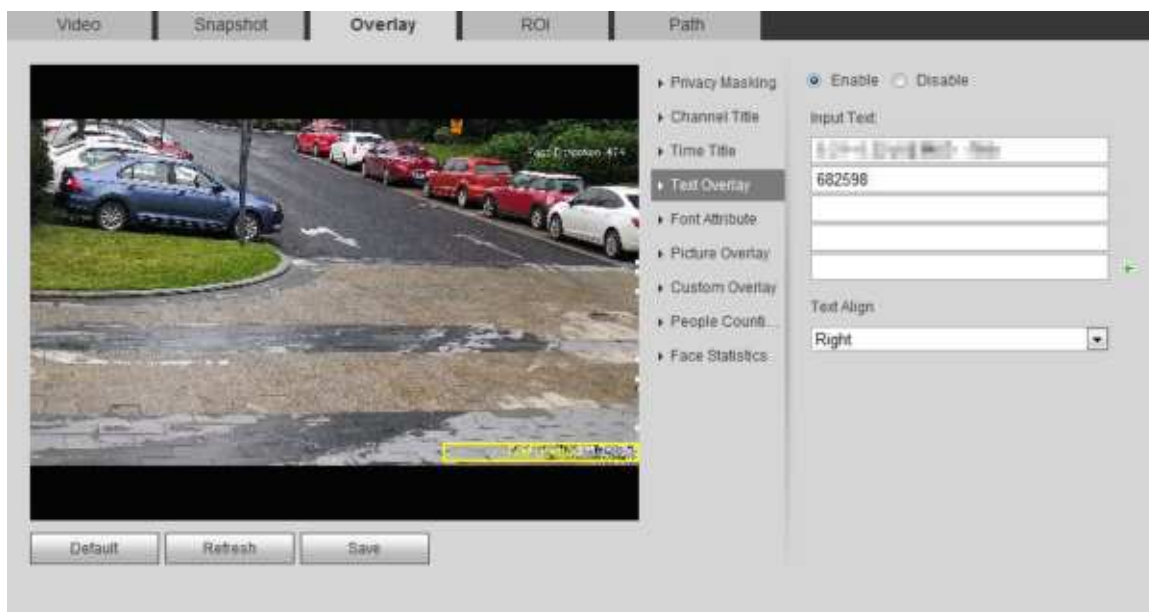
Figure 4-60 Text overlay
