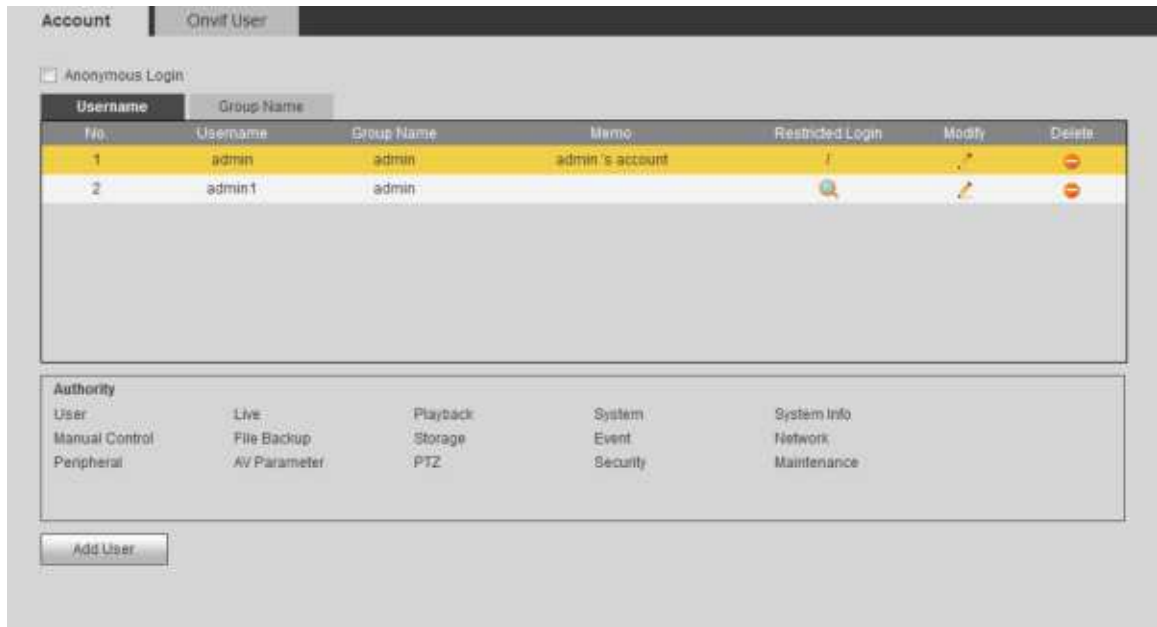
Figure 4-102 Username
