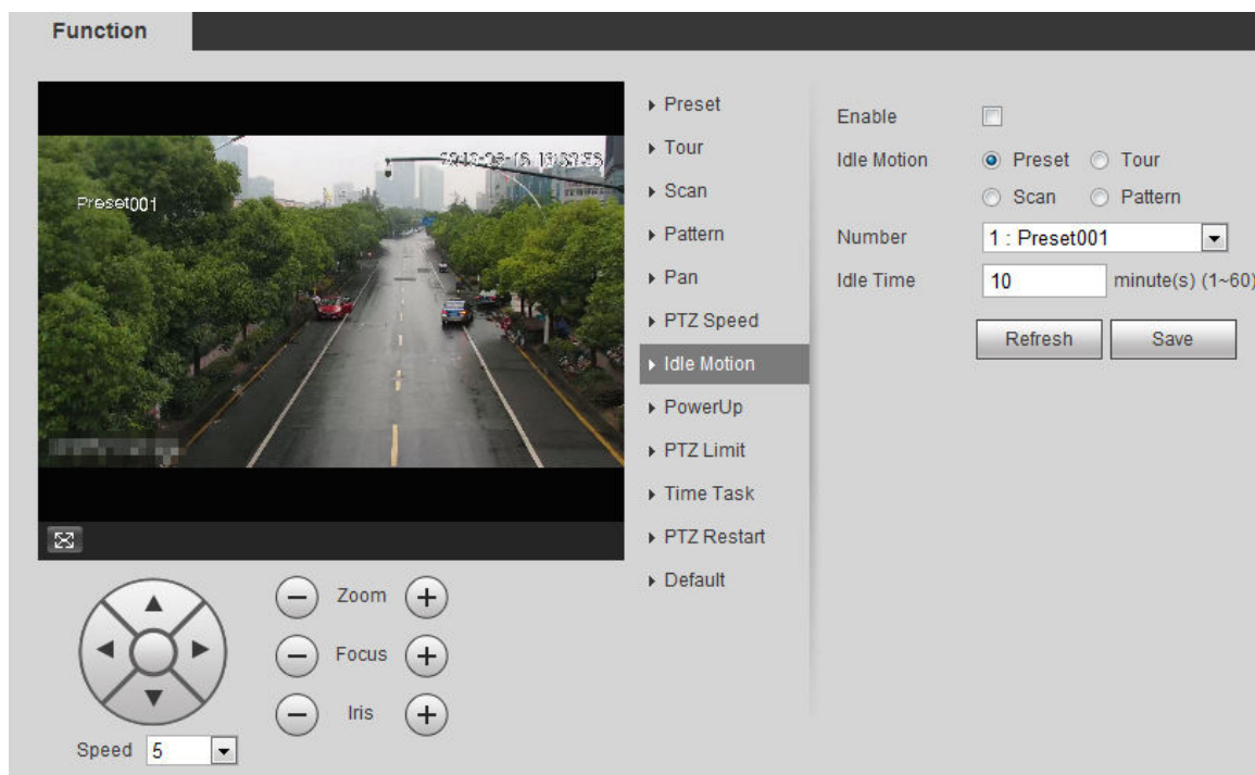
Figure 4-14 Idle motion
