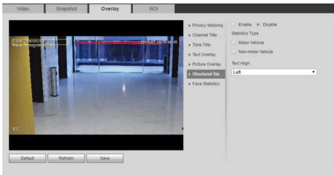
Figure 4-66 Structured statistics
