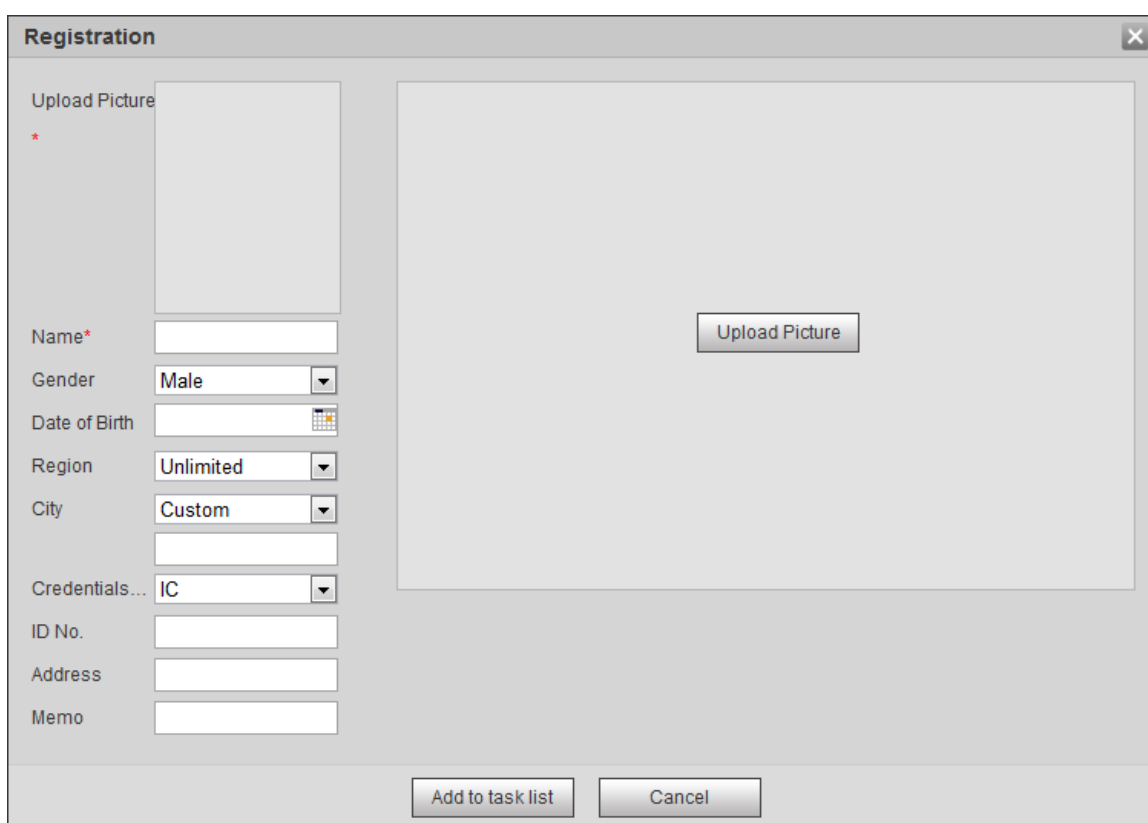
Figure 5-45 Registration (1)
