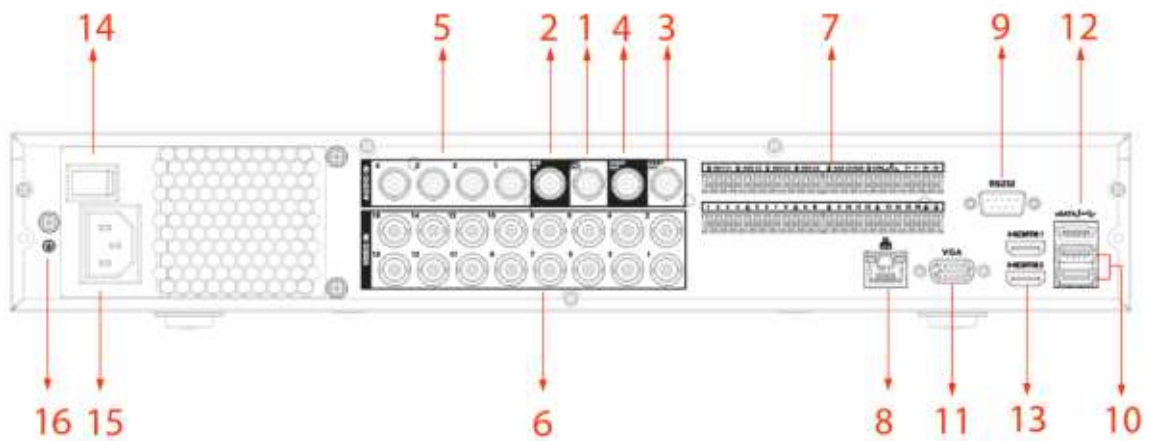
Figure 3-20 Rear panel (3)
