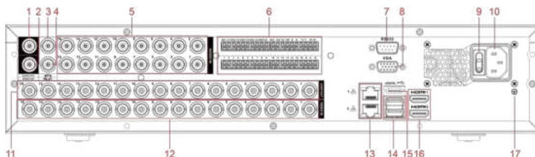
Figure 3-17 Rear panel
