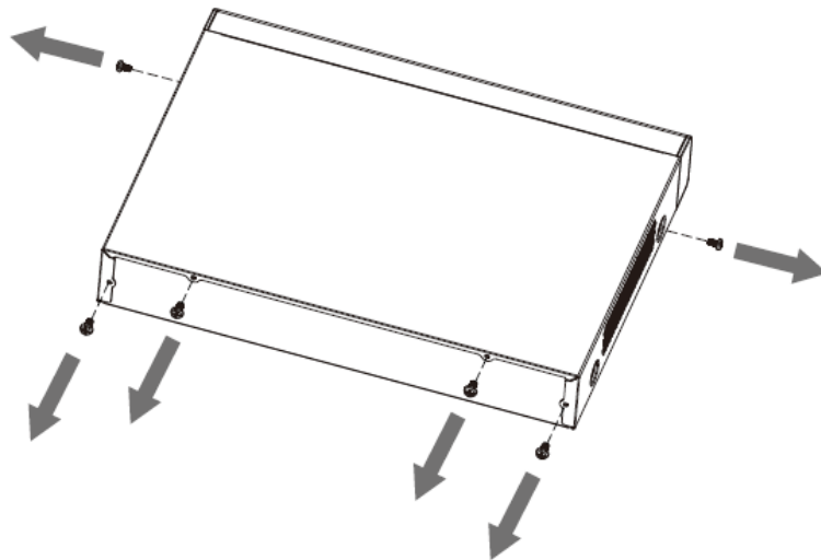
Figure 2-24 Remove screws
