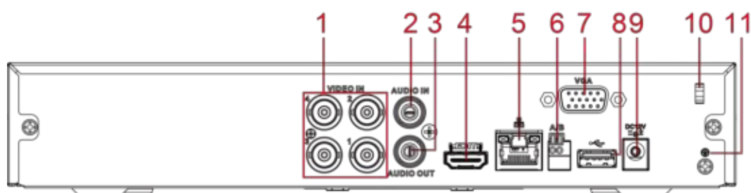
Figure 3-13 Rear panel
