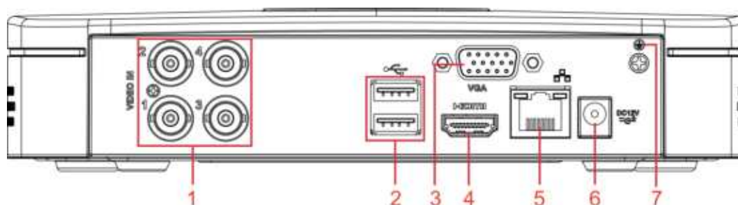
Figure 3-22 Rear panel
