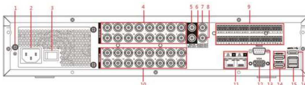
Figure 3-16 Rear panel
