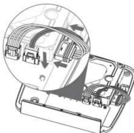
Figure 2-33 Connect cables
