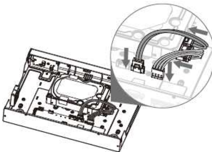
Figure 2-27 Connect cables
