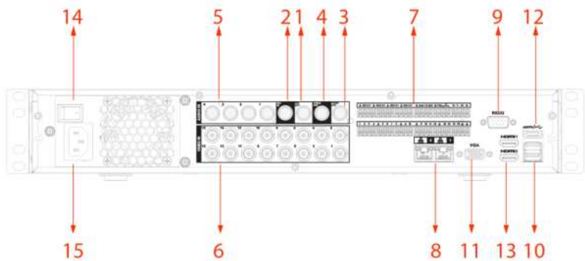
Figure 3-20 Rear panel (3)
