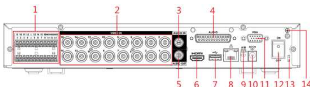
Figure 3-12 Rear panel
