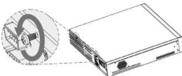
Figure 2-7 Remove screws
