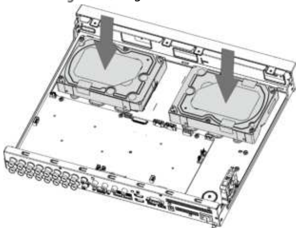
Figure 2-3 Align screws
