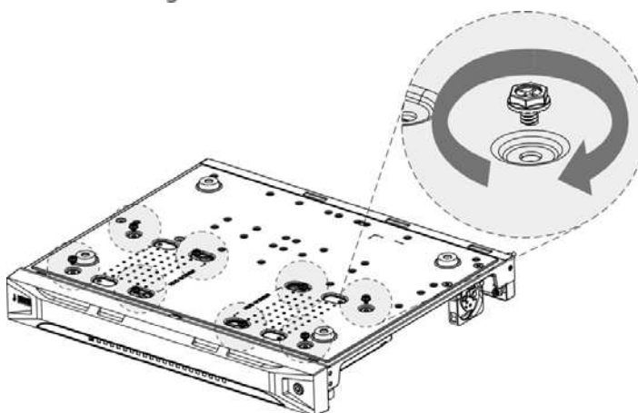
Figure 2-4 Fasten screws
