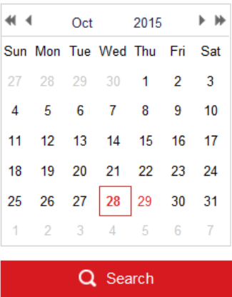
Figure 7-2 Search Video
