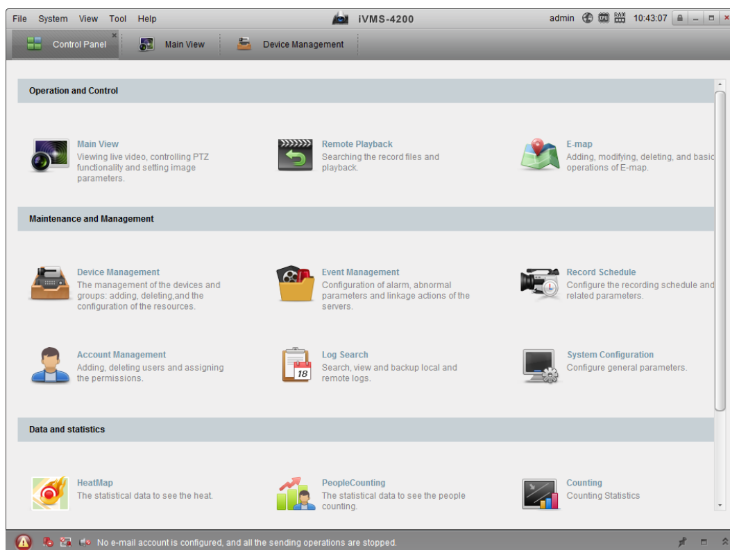
Figure 2-6 Control Panel
