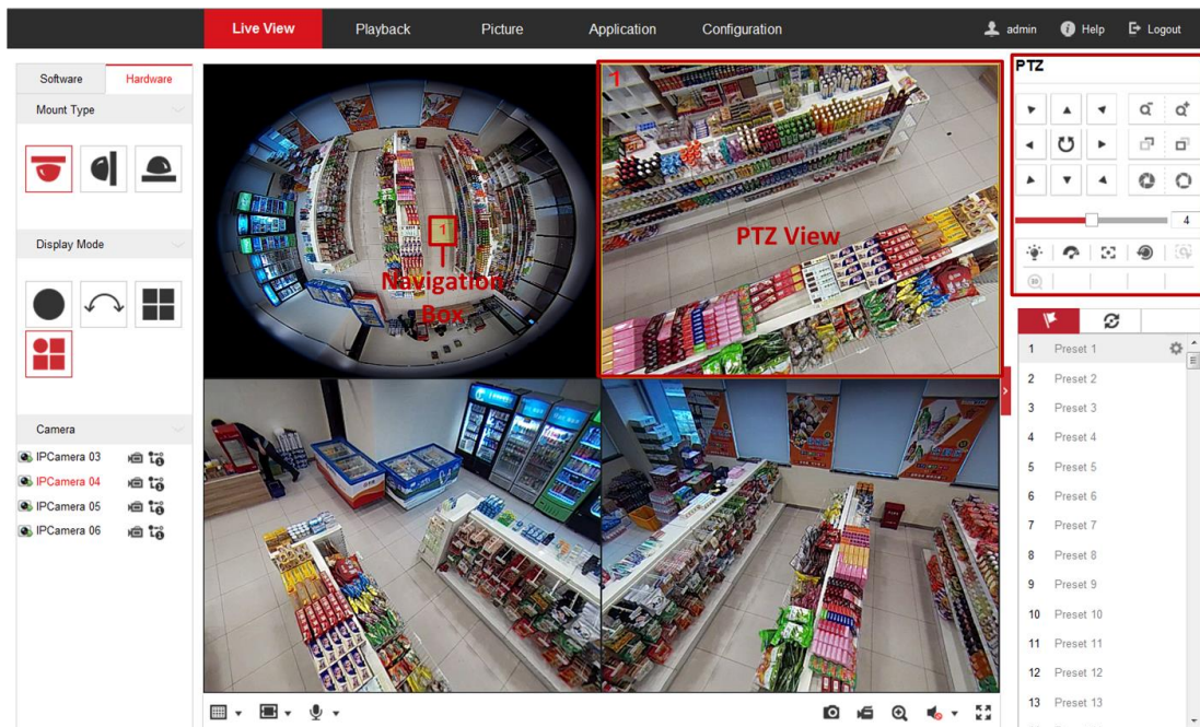
Figure 4-5 PTZ Control
