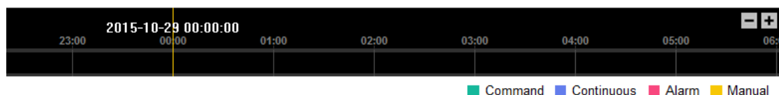
Figure 7-6 Progress Bar
