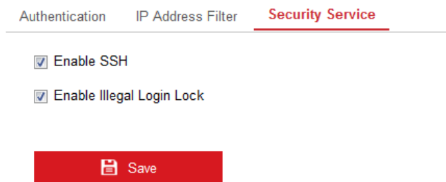
Figure 5-16 Security Service
