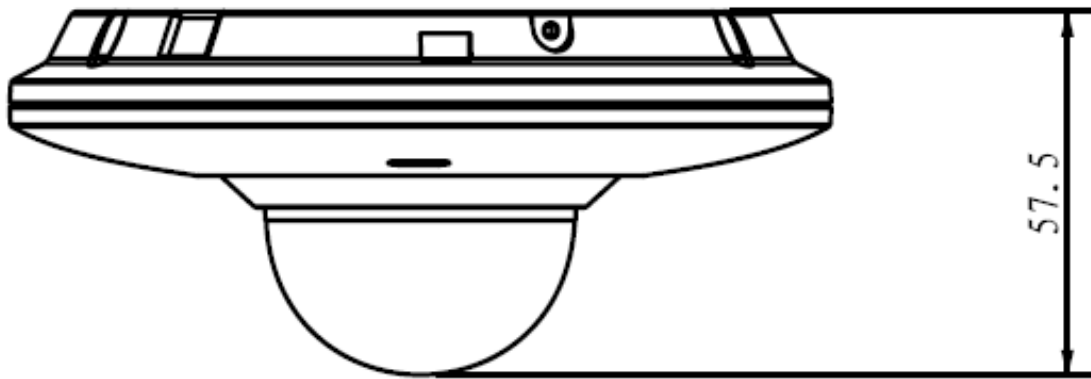
Figure 2-2 Dimension illustration 1
