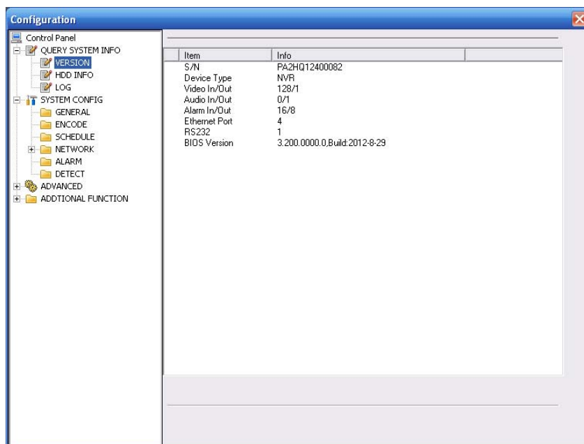
Figure 5-14 Version Information
