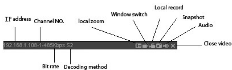
Figure 5-6 Real-time Monitor
