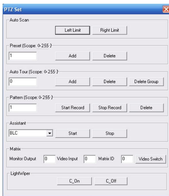
Figure 5-11 PTZ Setup
