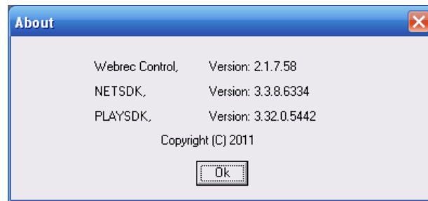
Figure 5-56 About
