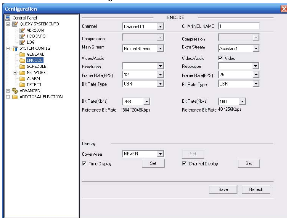
Figure 5-20 Encode
