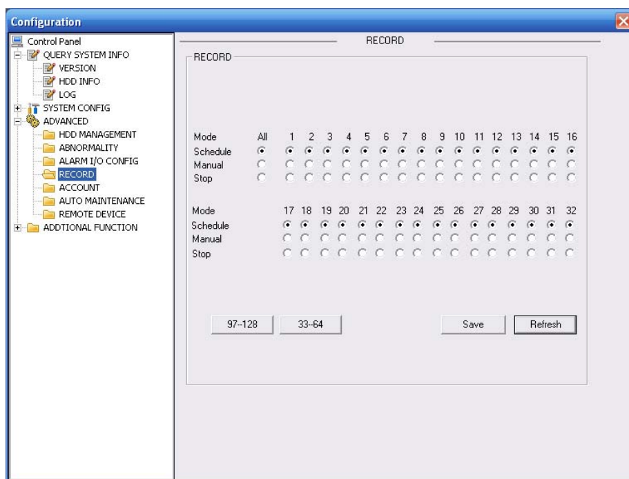
Figure 5-43 Record
