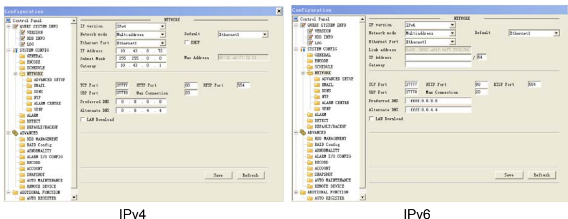
Figure 5-25 Network
