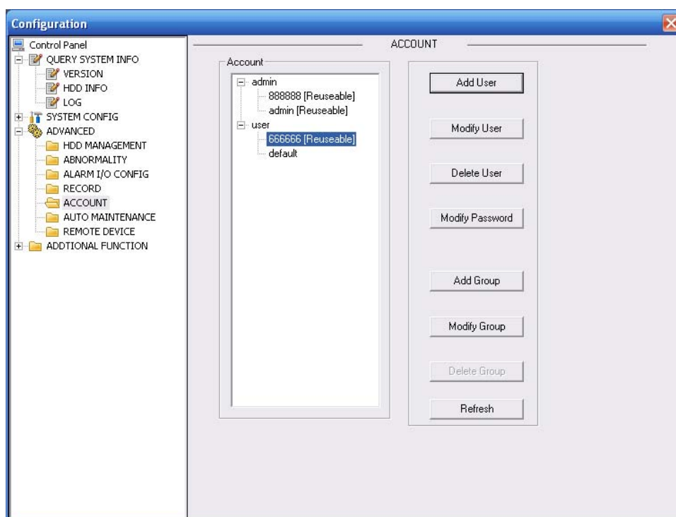
Figure 5-44 Account
