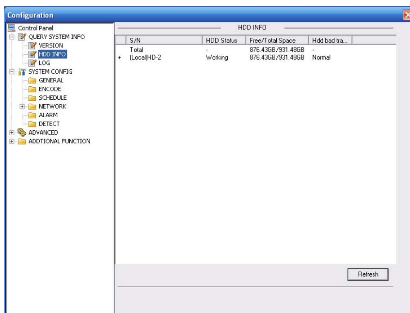
Figure 5-15 HDD Information
