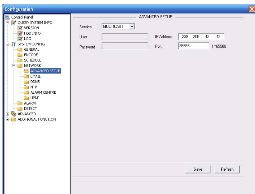
Figure 5-26 Network
