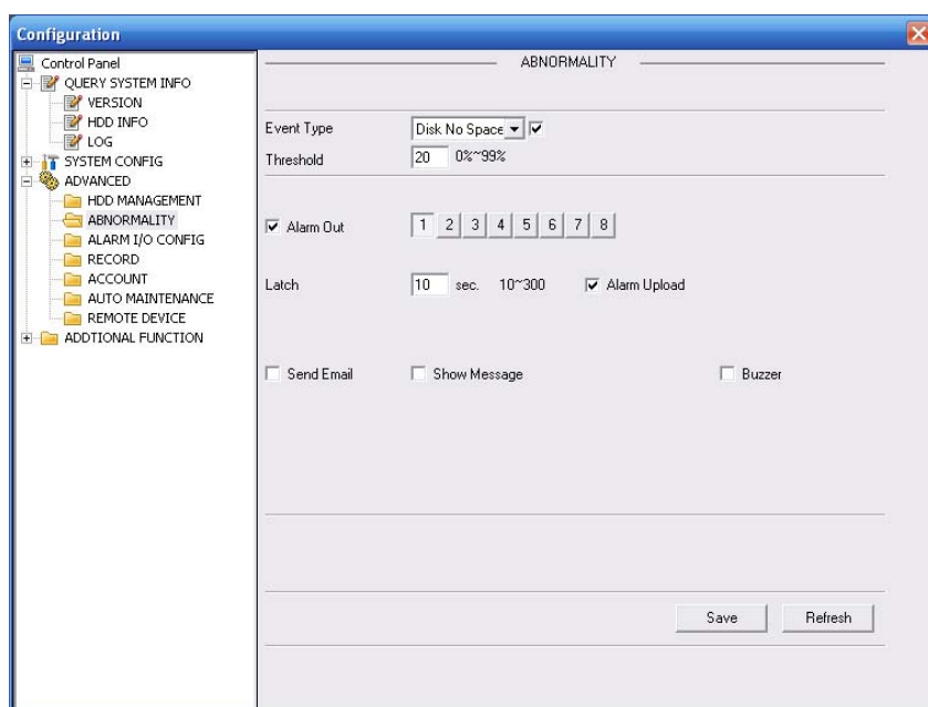
Figure 5-41 Abnormality -2
