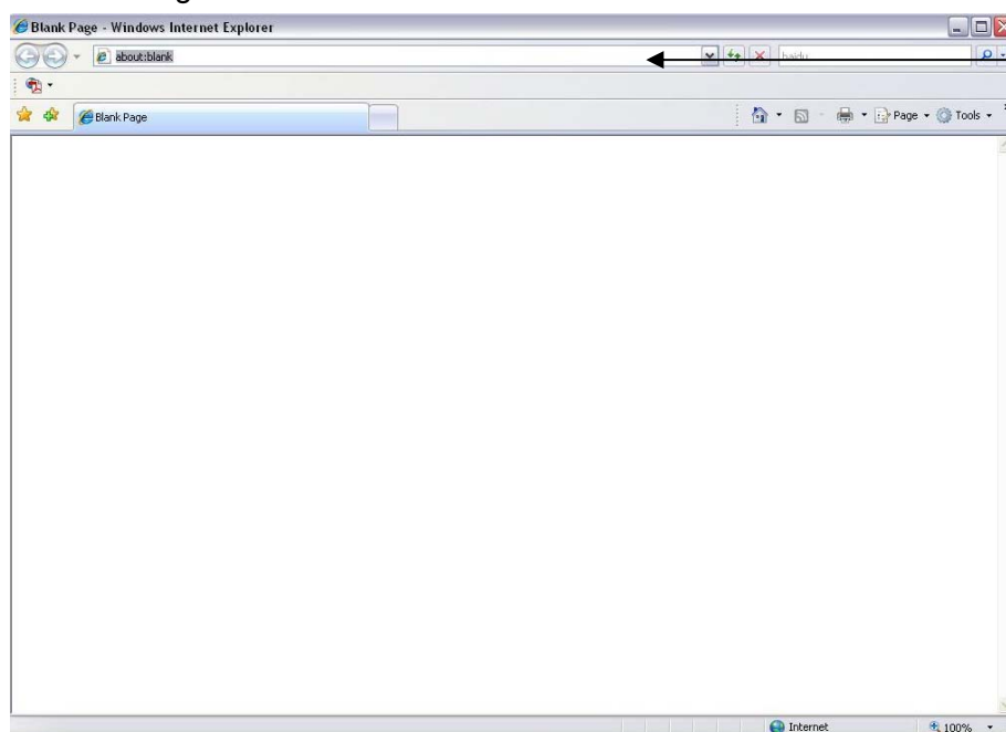
Figure 5-1 IE Interface
