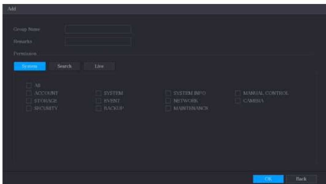
Figure 5-302 Add group
