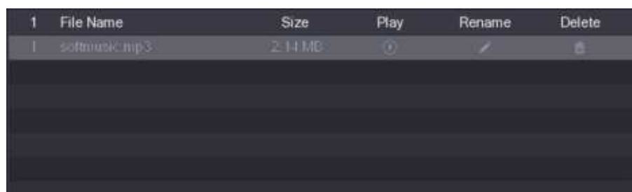
Figure 5-310 Imported file
