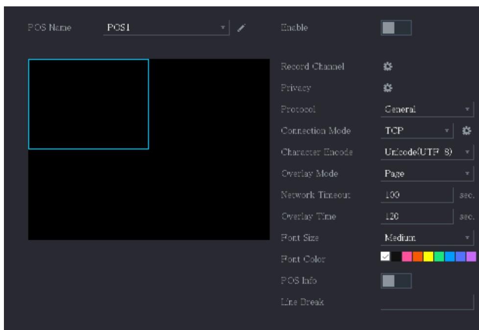
Figure 5-271 POS setting
