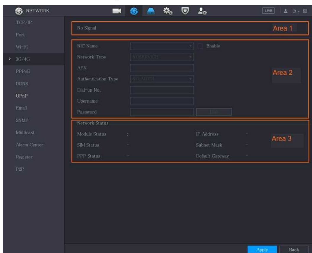
Figure 5-278 3G/4G
