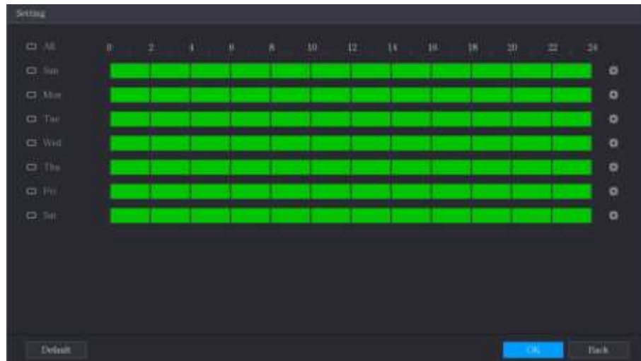
Figure 5-296 Setting
