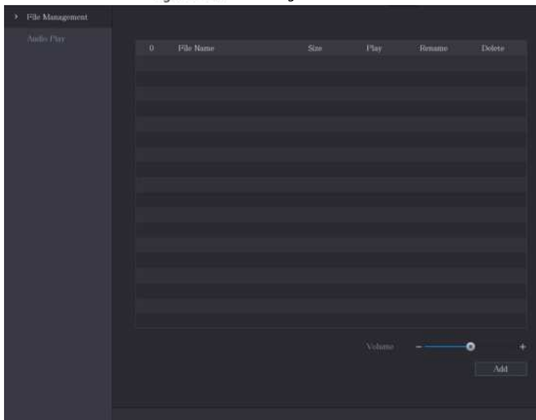
Figure 5-308 File management
