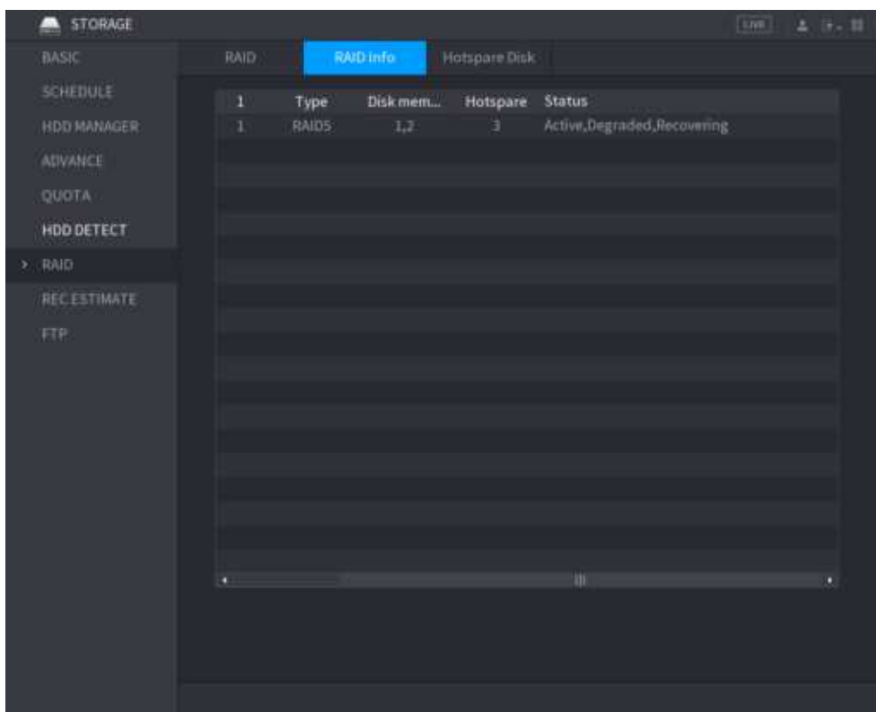
Figure 5-265 RAID info
