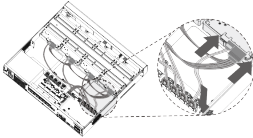
Figure 2-22 Connect cables
