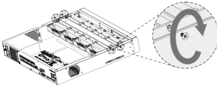
Figure 2-21 Fasten screws
