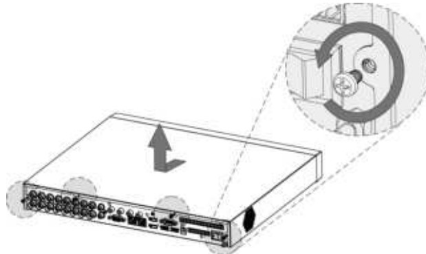
Figure 2-1 Remove screws
