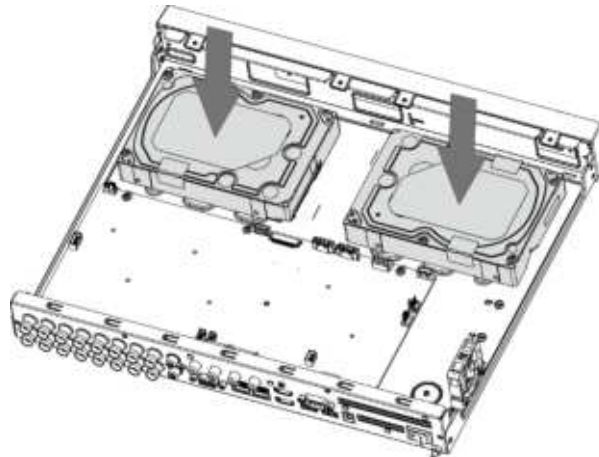
Figure 2-3 Align screws
