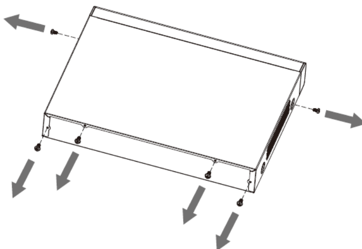
Figure 2-24 Remove screws
