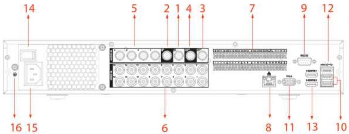
Figure 3-20 Rear panel (3)
