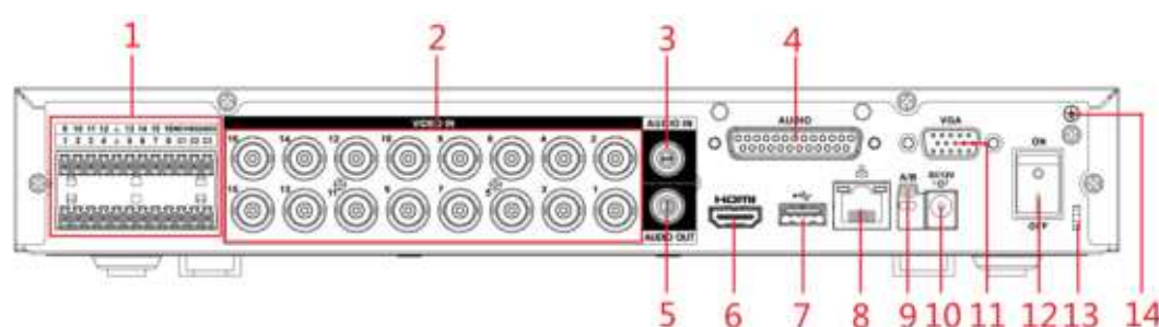
Figure 3-12 Rear panel
