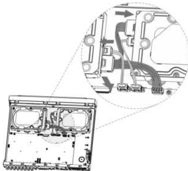
Figure 2-5 Connect cables
