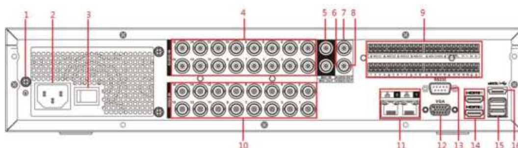
Figure 3-16 Rear panel
