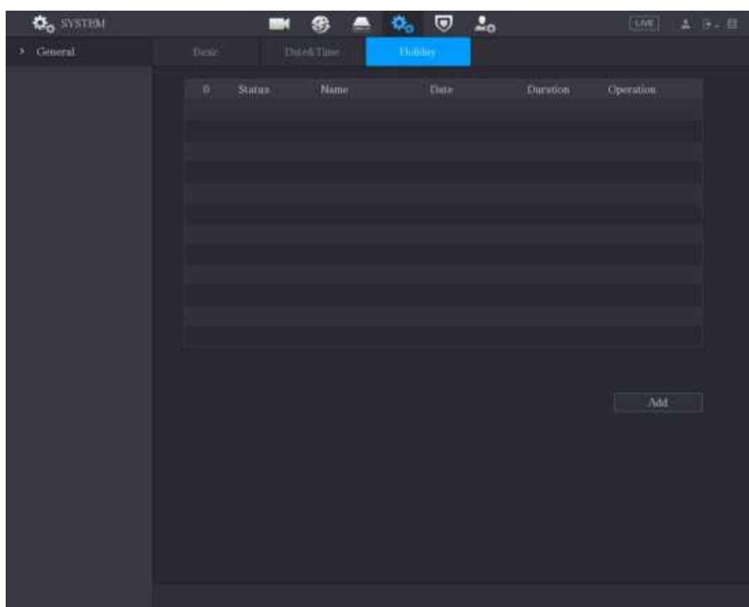
Figure 5-339 Holiday
