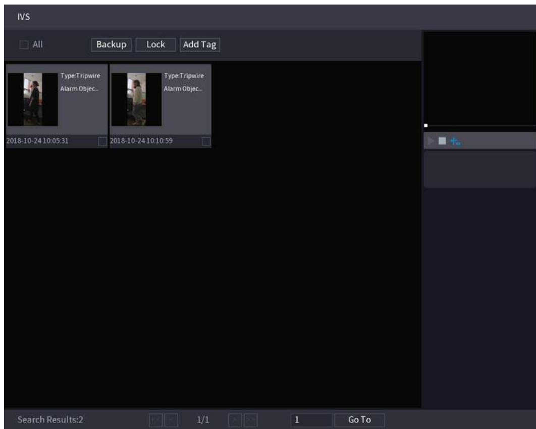
Figure 5-186 Search results
