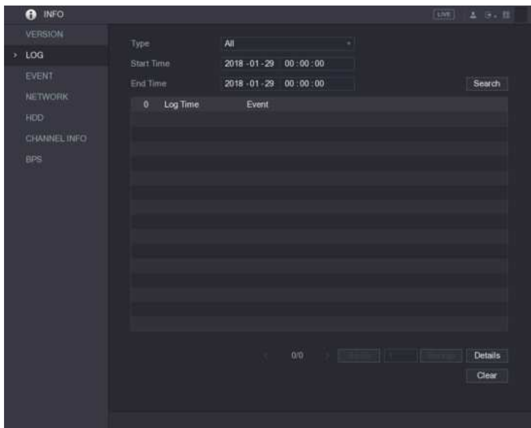
Figure 5-351 Log
