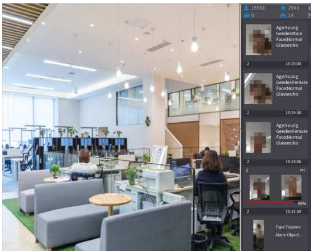
Figure 5-44 Live view
