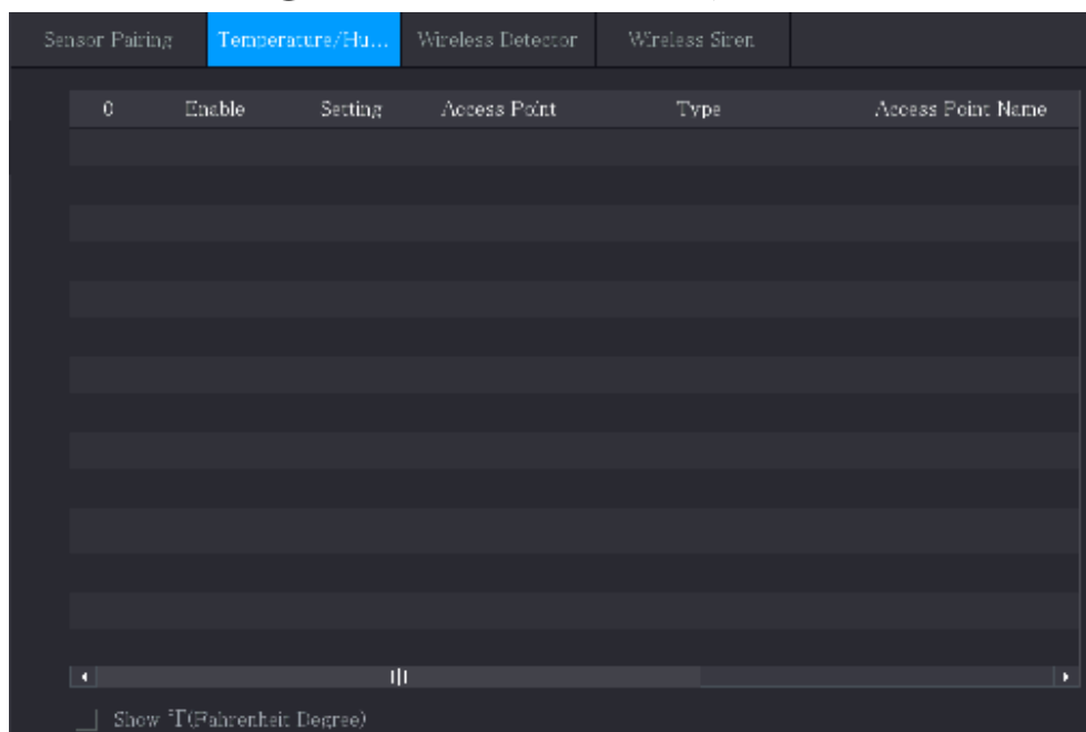
Figure 5-251 Temperature/Humidity
