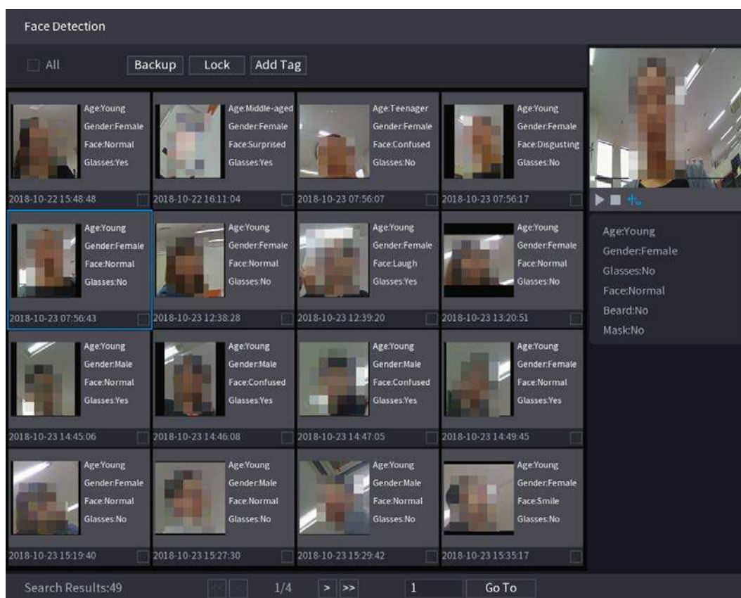
Figure 5-212 Registered information
