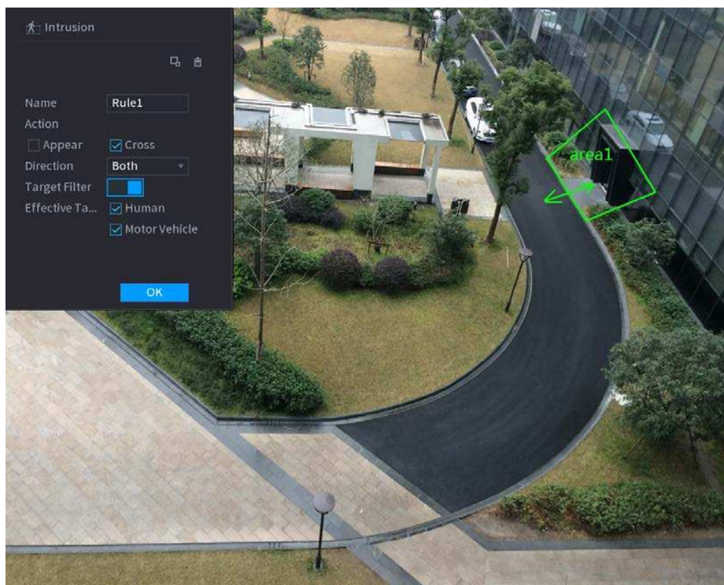
Figure 5-183 Intrusion rule
