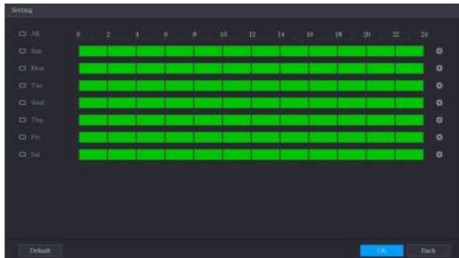
Figure 5-289 Setting
