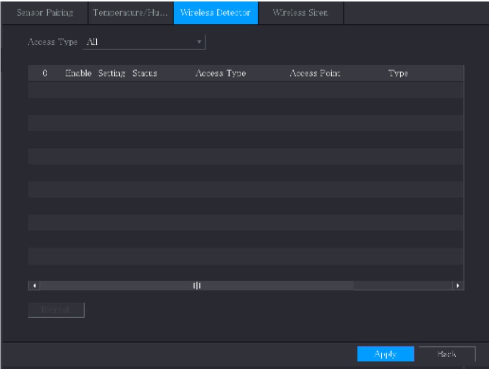
Figure 5-249 Wireless detector
