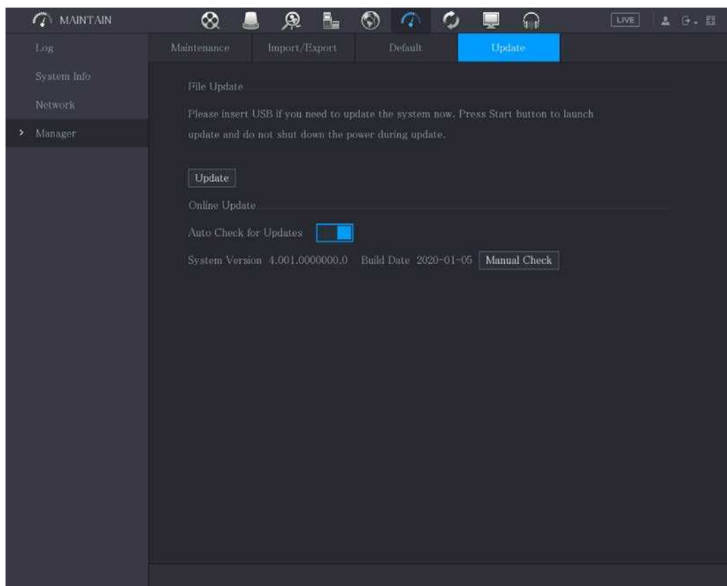
Figure 5-347 Update
