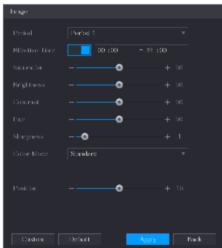
Figure 5-48 Image
