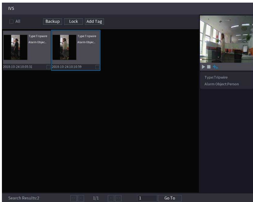
Figure 5-187 Playback
