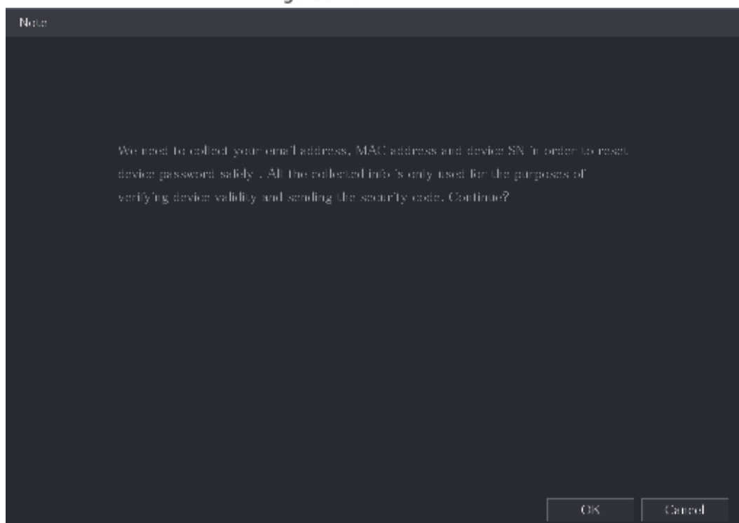
Figure 5-10 Note
