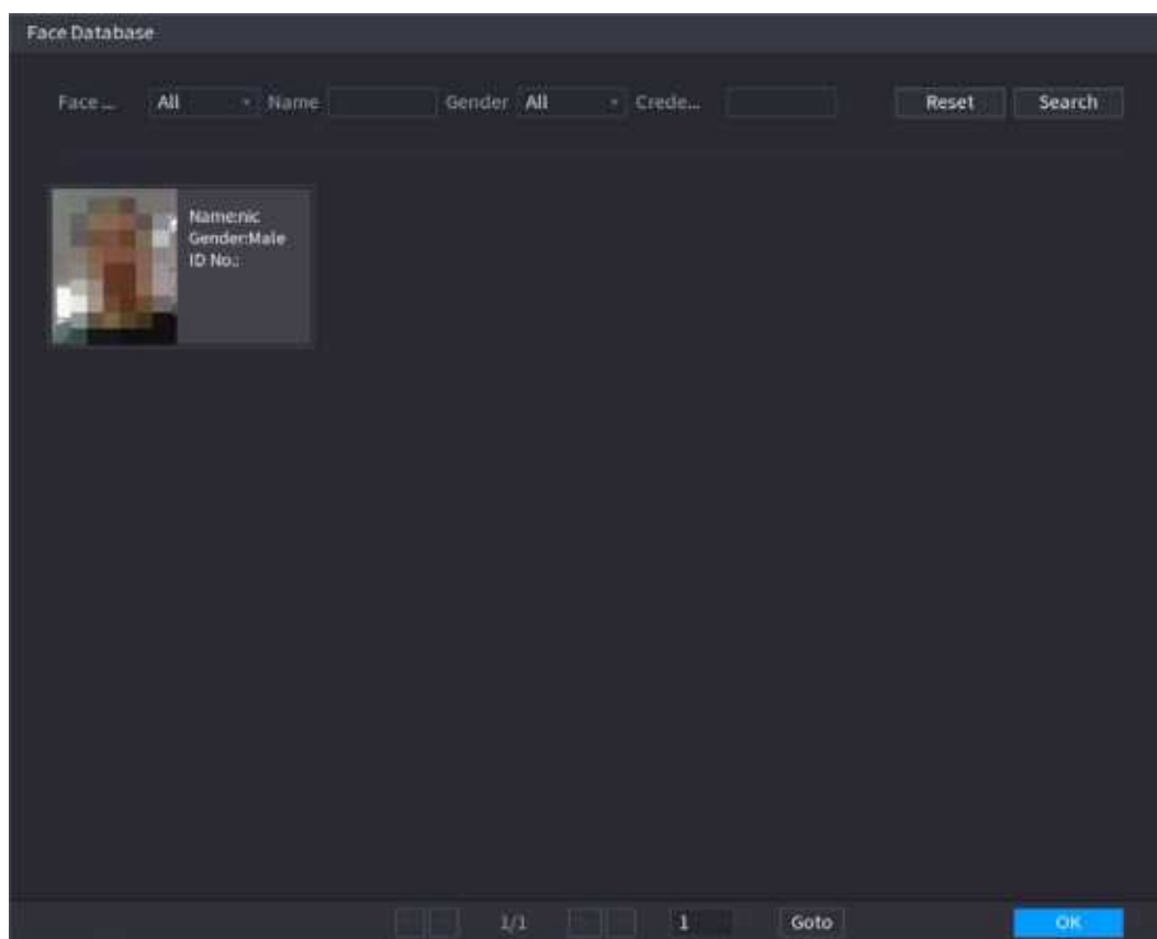
Figure 5-170 Face database
