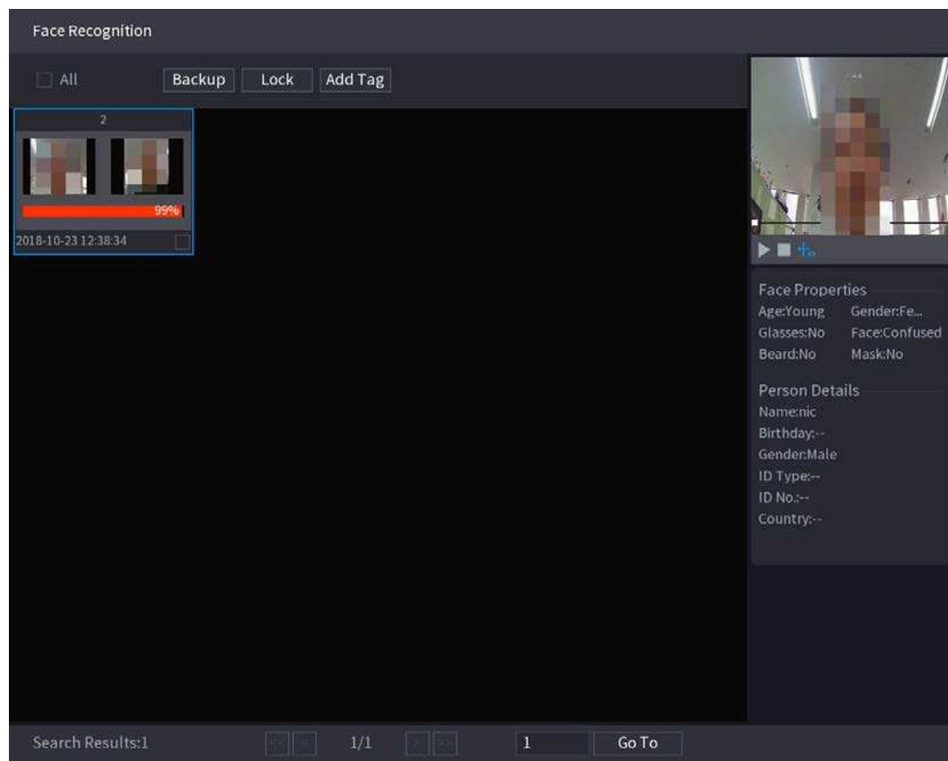
Figure 5-167 Registered information
