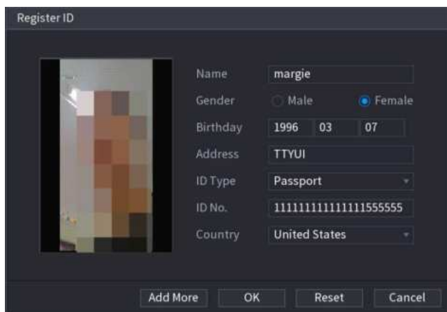
Figure 5-155 Register ID
