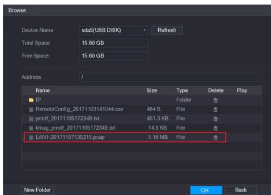
Figure 5-286 Backup data
