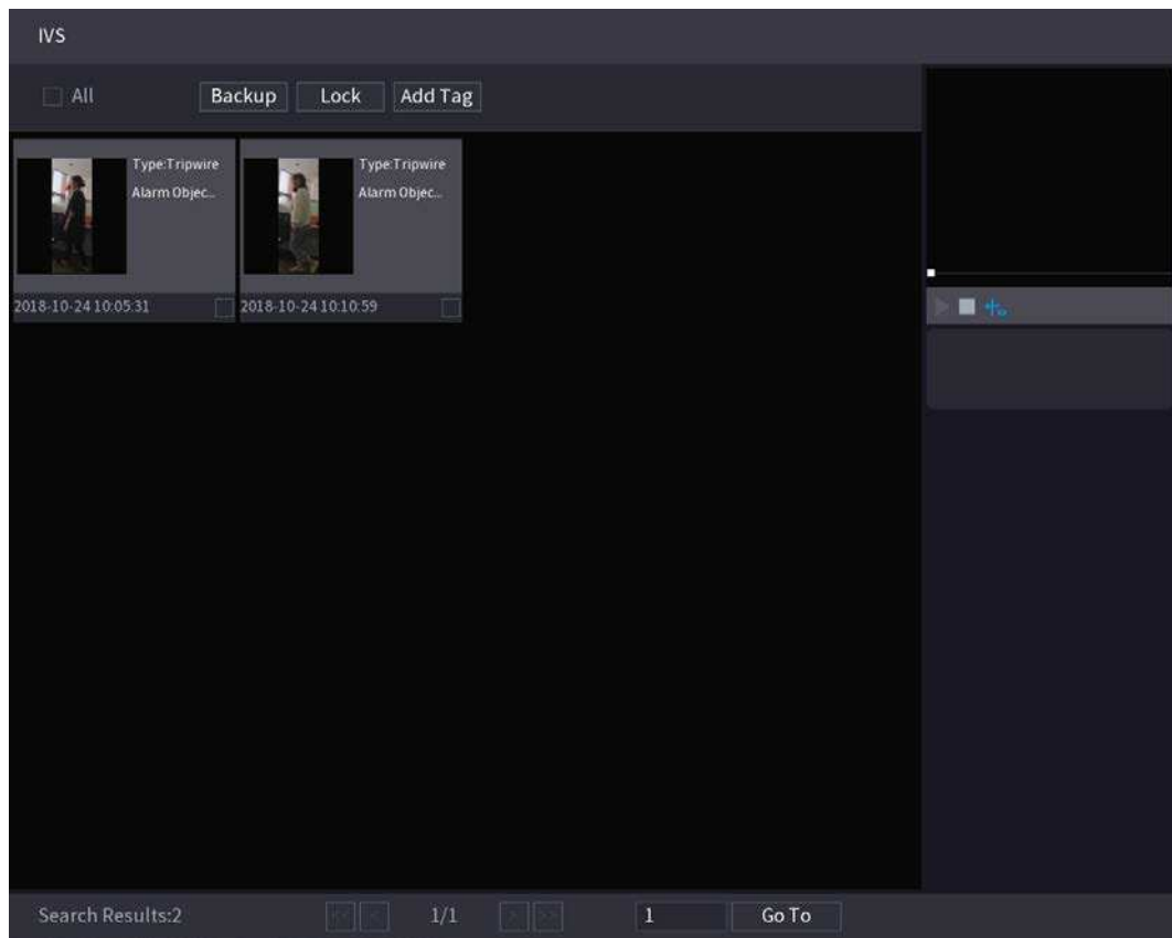
Figure 5-206 Search results
