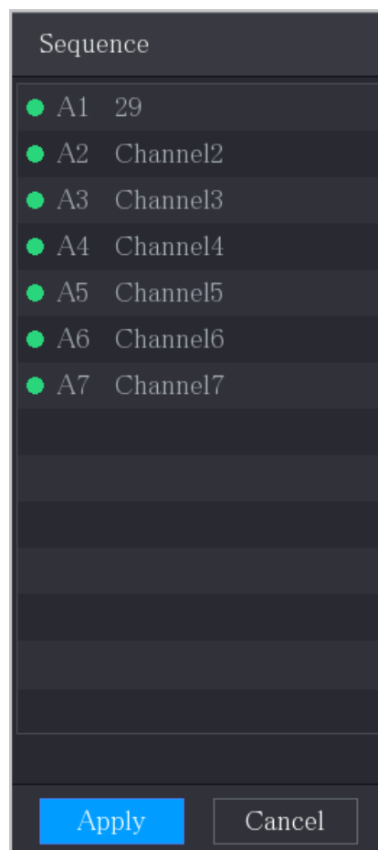
Figure 5-46 Sequence
