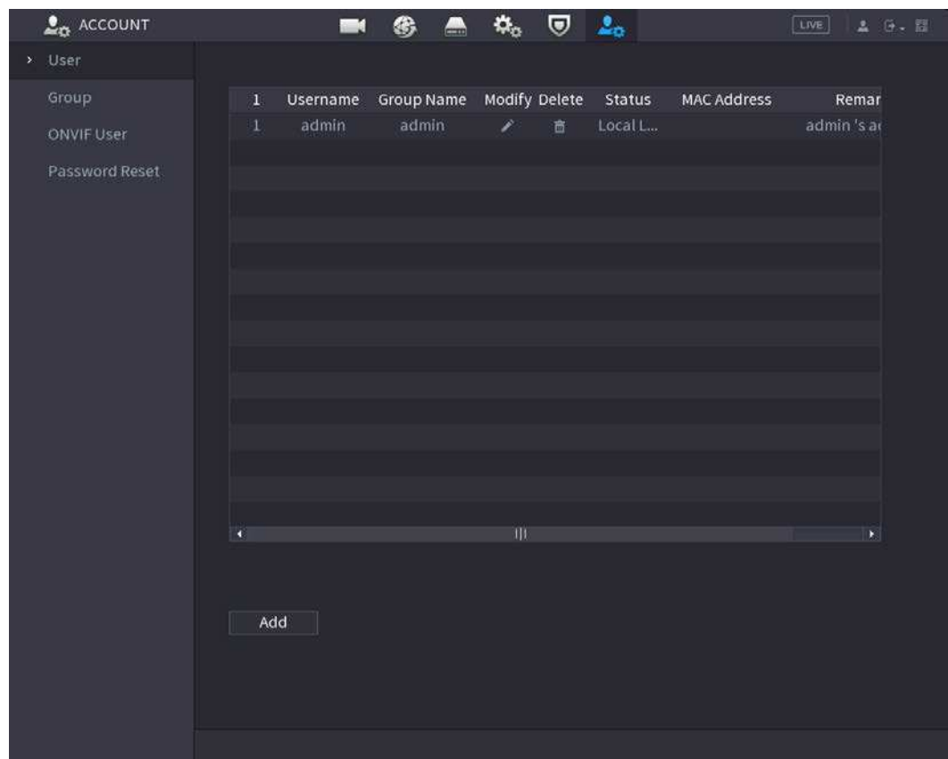
Figure 5-291 User
