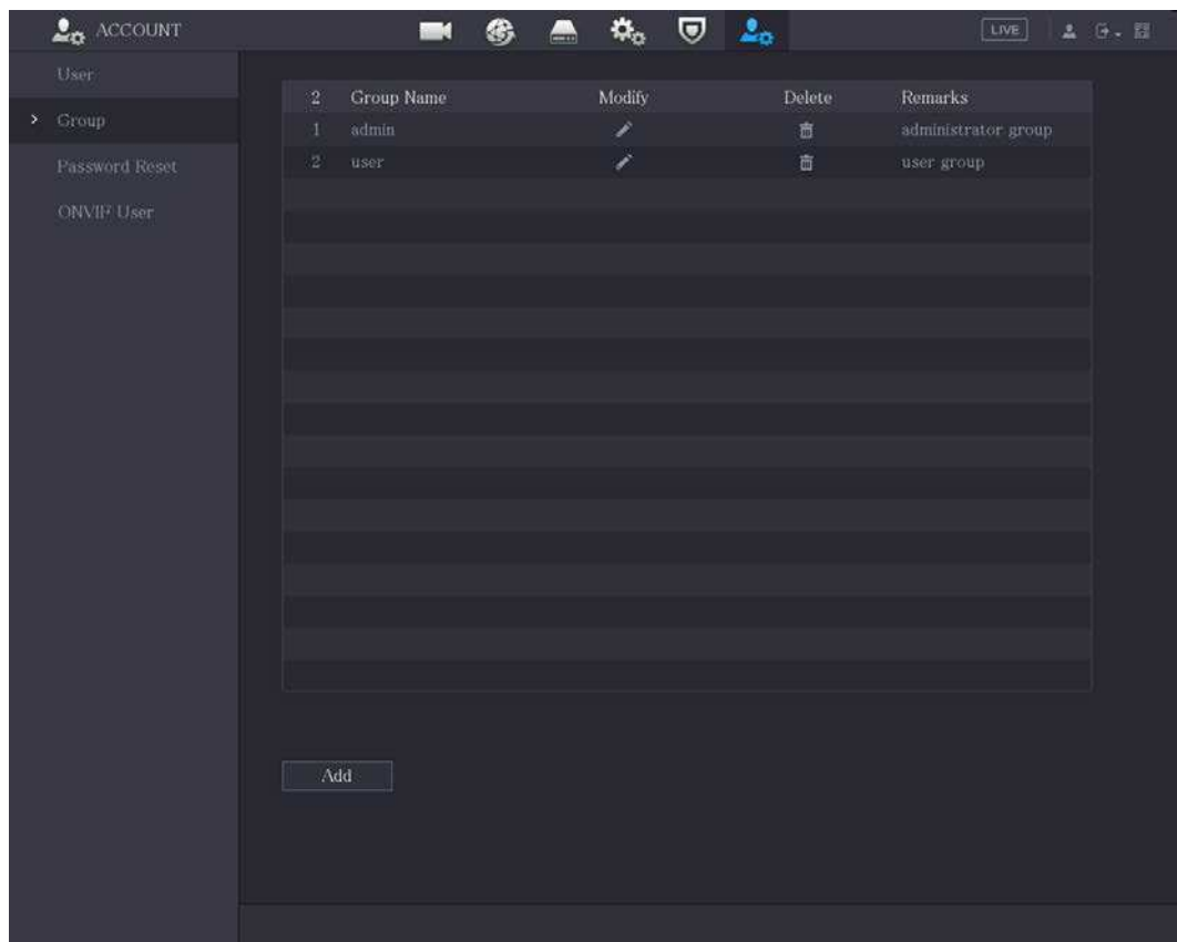
Figure 5-294 Group
