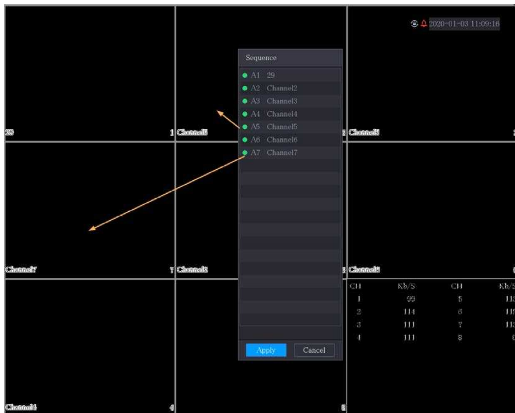
Figure 5-47 Adjusted sequence
