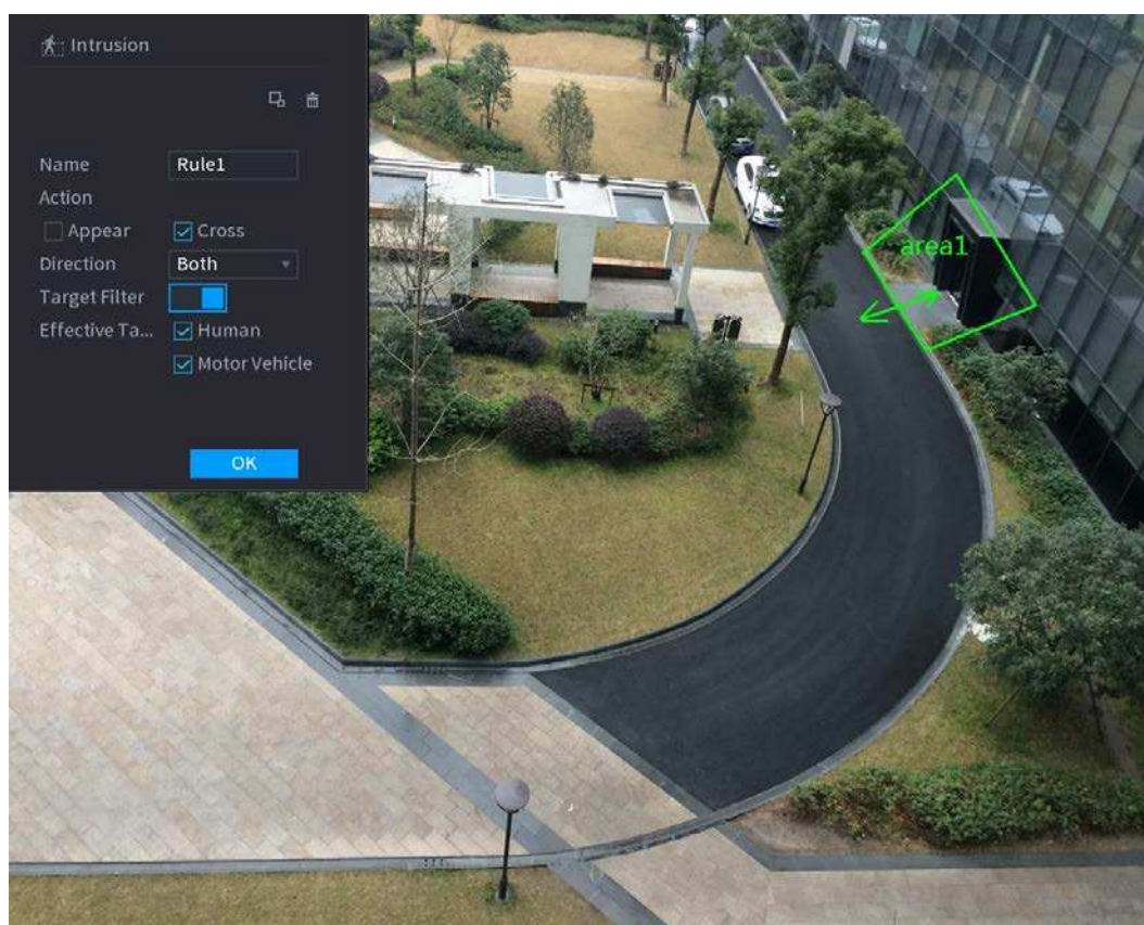
Figure 5-204 Intrusion rule
