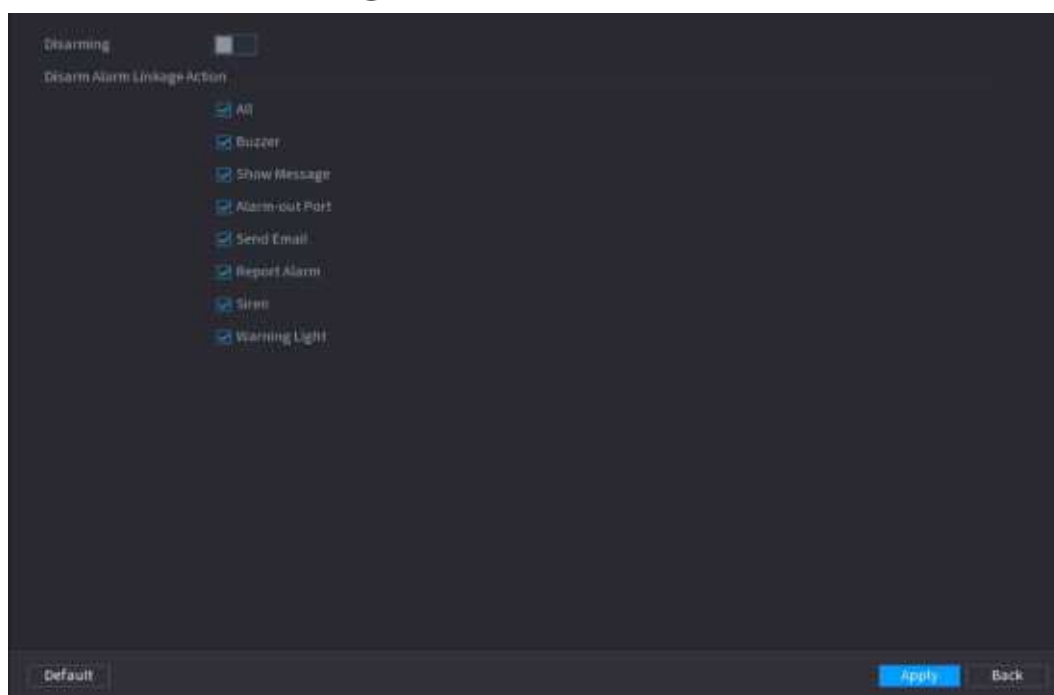
Figure 5-142 Disarming
