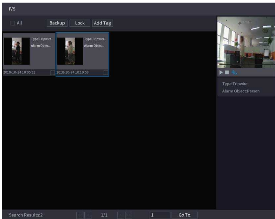
Figure 5-207 Playback
