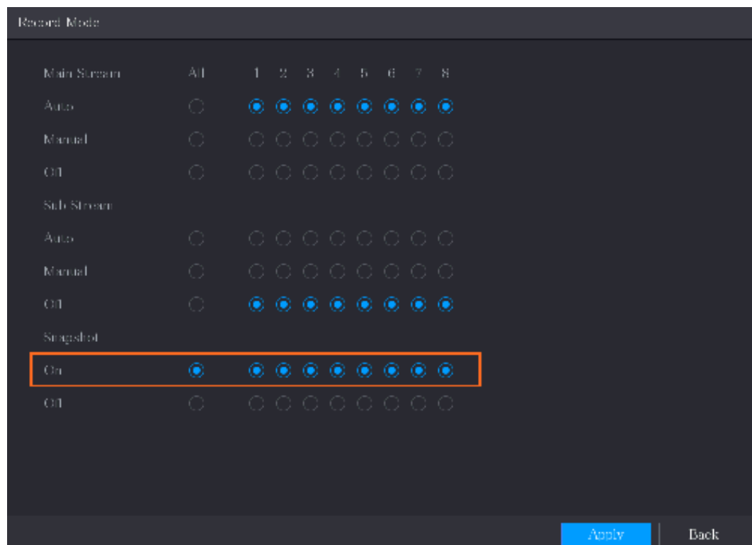
Figure 5-103 Enable snapshot
