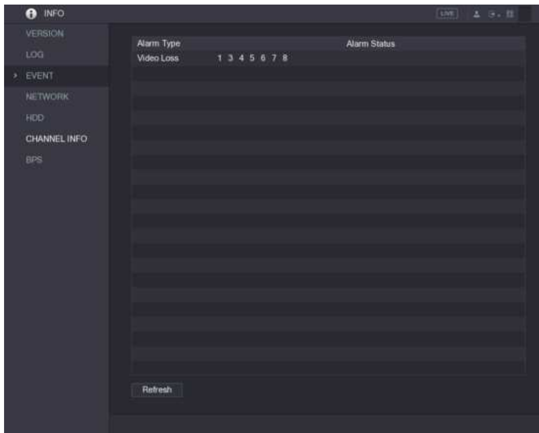
Figure 5-353 Event
