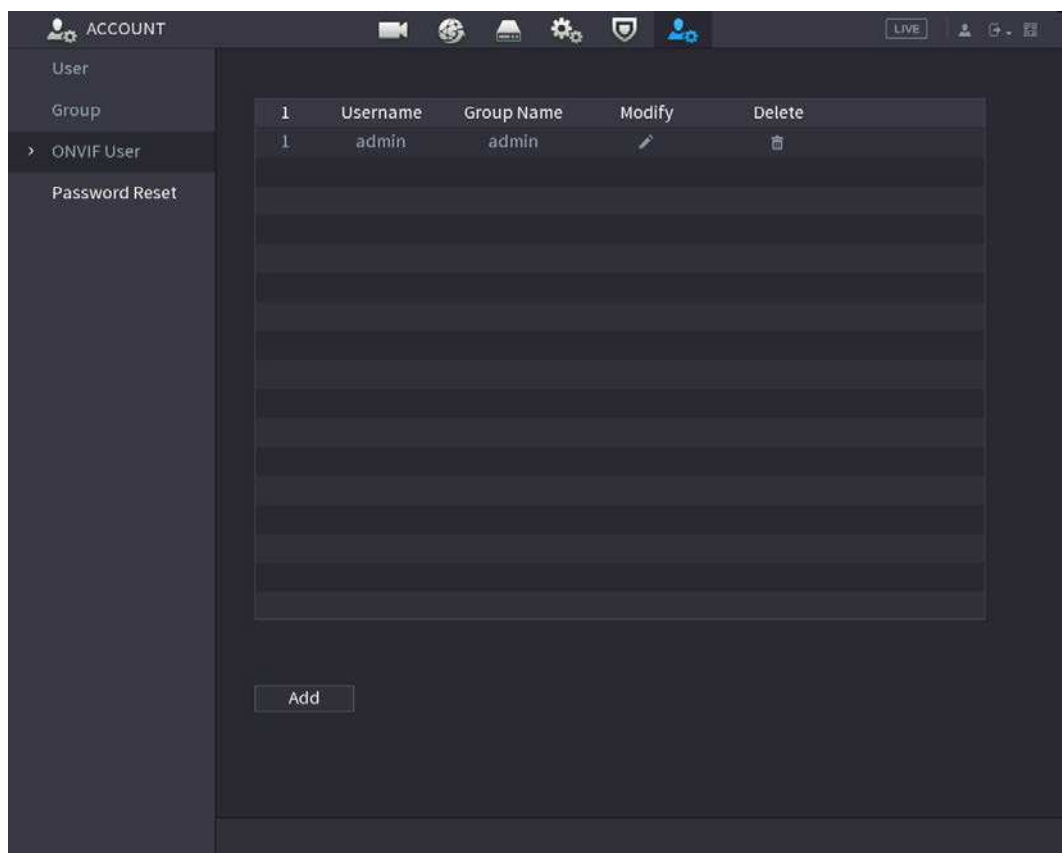
Figure 5-299 ONVIF user
