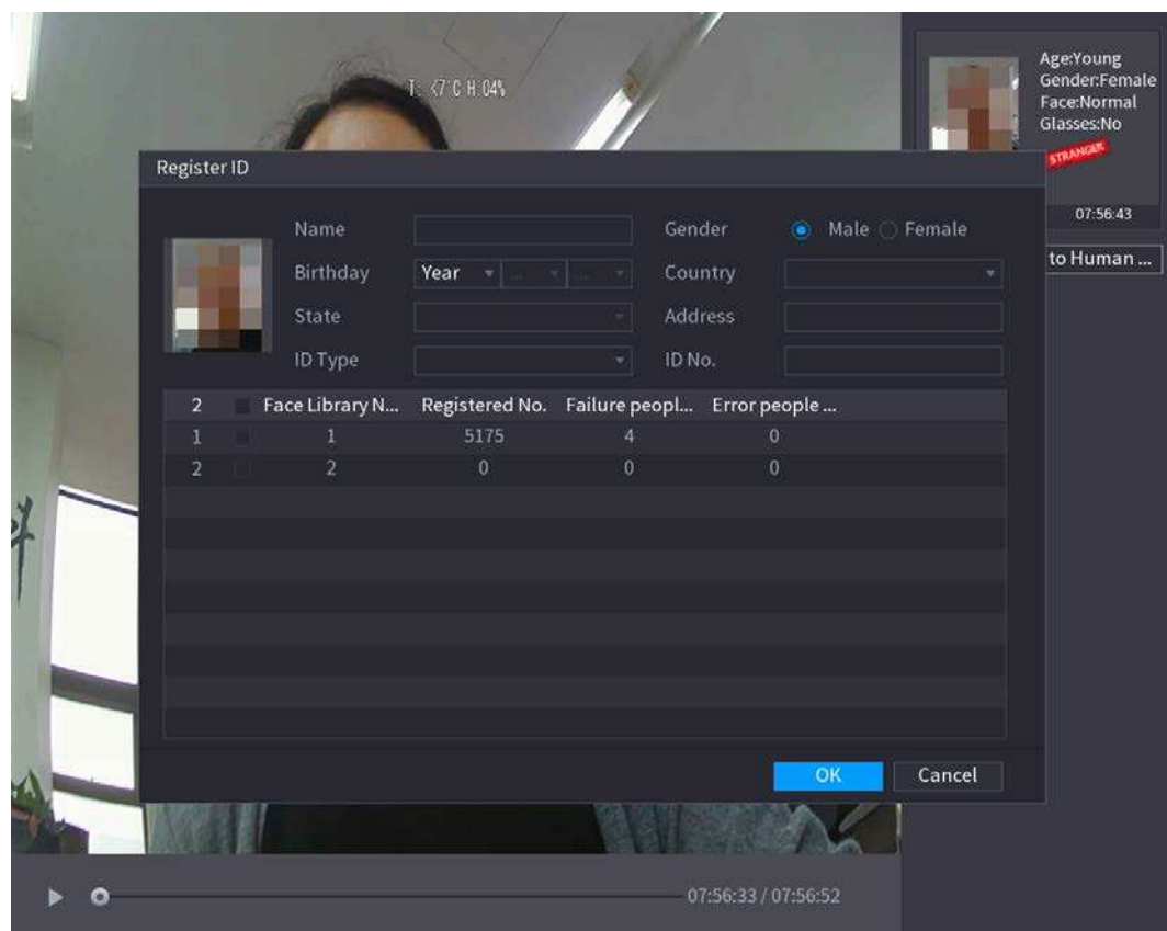
Figure 5-226 Register ID
