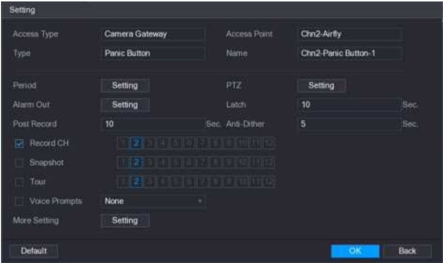
Figure 5-250 Setting
