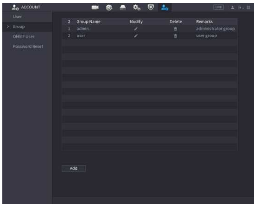
Figure 5-296 Group
