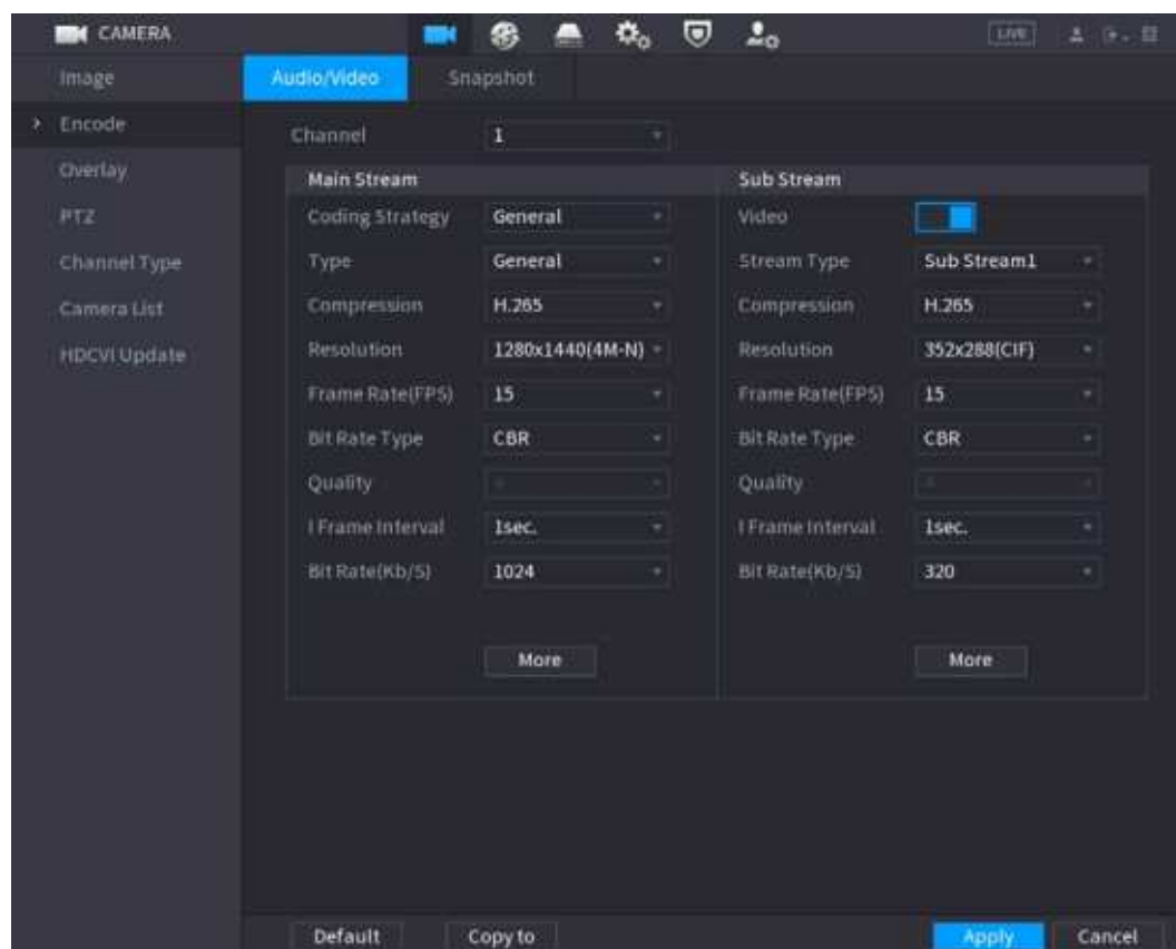
Figure 5-75 Audio/video
