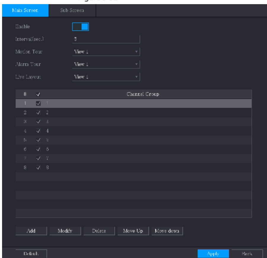
Figure 5-52 Main screen
