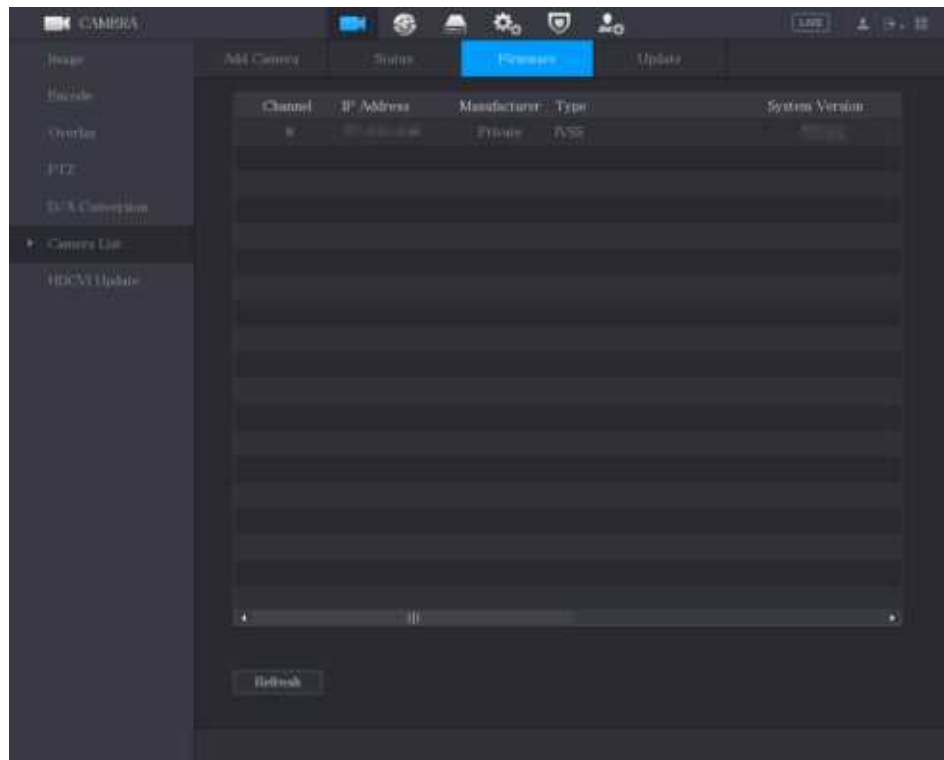
Figure 5-100 Firmware
