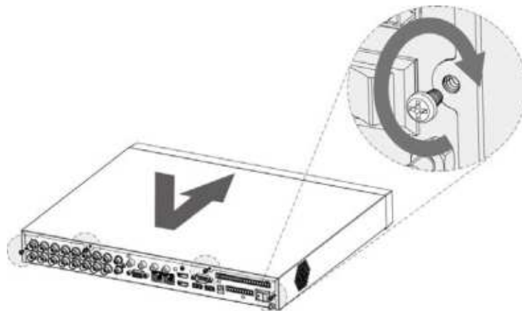
Figure 1-6 Installation completed
