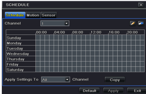
Fig 4-14 Schedule Configuration-Schedule
