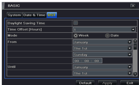
Fig 4-5 Basic Configuration-DST
