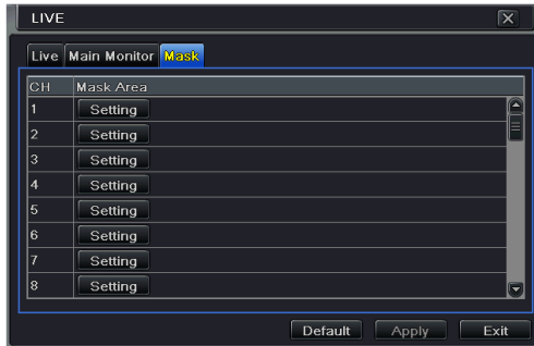
Fig 4-8 Live Configuration-Mask
