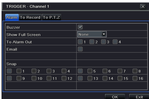
Fig 4-18 Alarm Handling-Trigger
