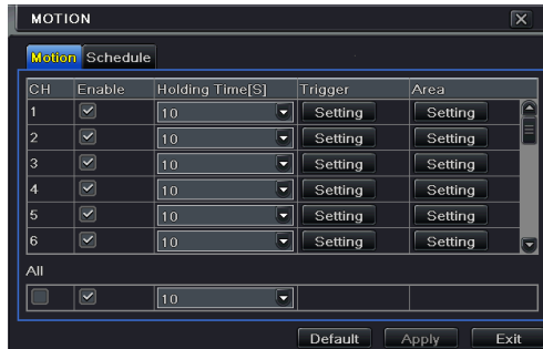
Fig 4-19 Alarm Configuration-Motion
