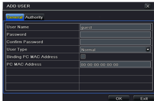
Fig 4-31 Add-General
