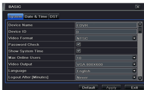
Fig 4-3 Basic Configuration-System
