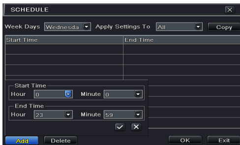
Fig 4-15 Schedule-Week Schedule
