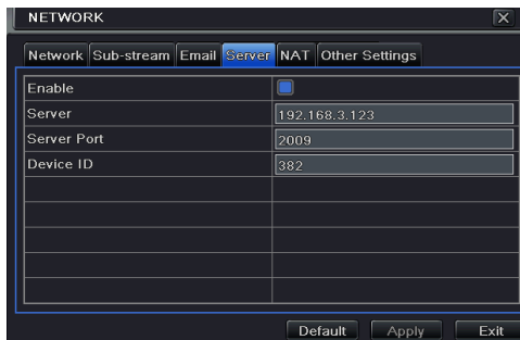
Fig 4-27 Network Configuration-Server
