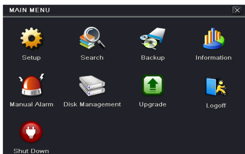
Fig 4-2 Main Menu
