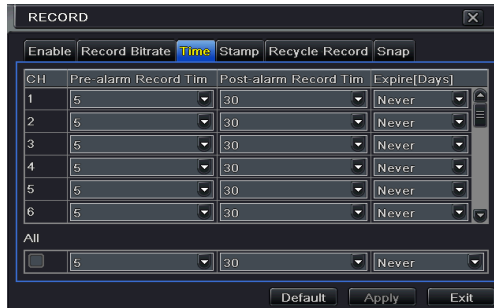
Fig 4-12 Record Configuration-Time
