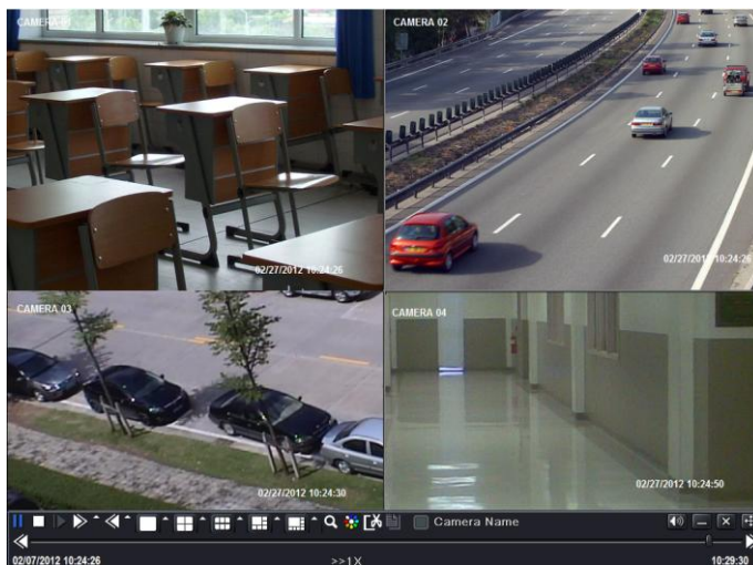
Fig 3-3 Live Playback
