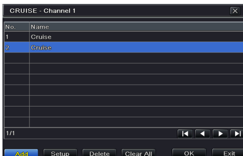
Fig 4-37 Cruise Setting
