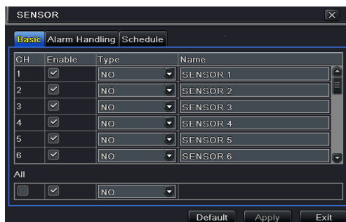
Fig 4-16 Alarm Configuration-Sensor-Basic
