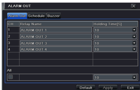
Fig 4-23 Alarm Out
