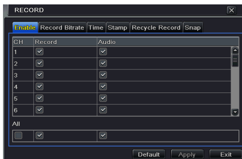
Fig 4-10 Record Configuration-Enable
