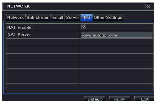
Fig 4-28 Network Configuration-NAT
