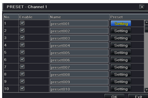
Fig 4-35 Advanced-Preset Setting
