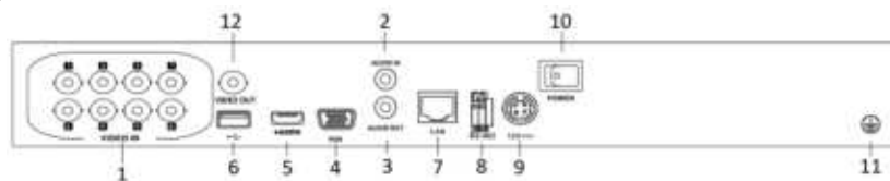
Figure 1. 10 Rear Panel 3
