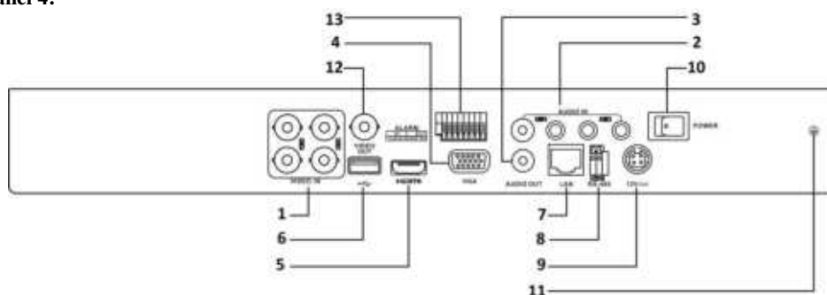
Figure 1. 11 Rear Panel 4
