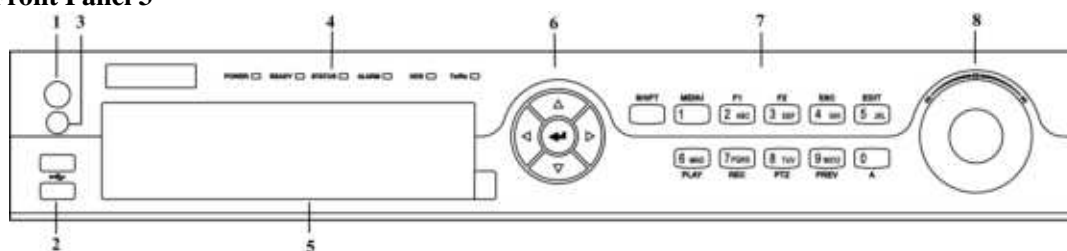
Figure 1. 3 Front Panel 3
