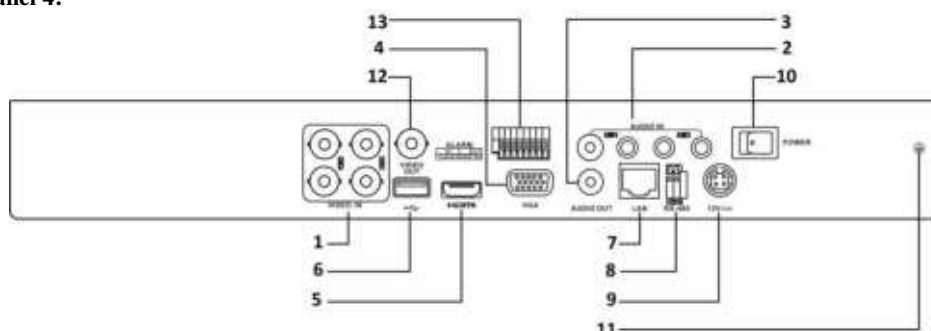
Figure 1. 11 Rear Panel 4
