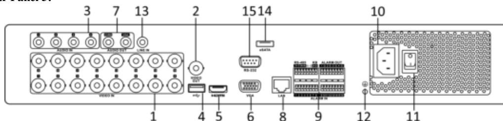
Figure 1. 12 Rear Panel 5
