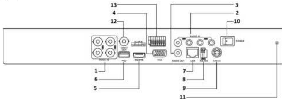
Figure 1. 11 Rear Panel 4
