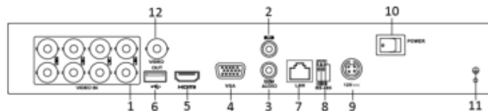
Figure 1. 9 Rear Panel 2
