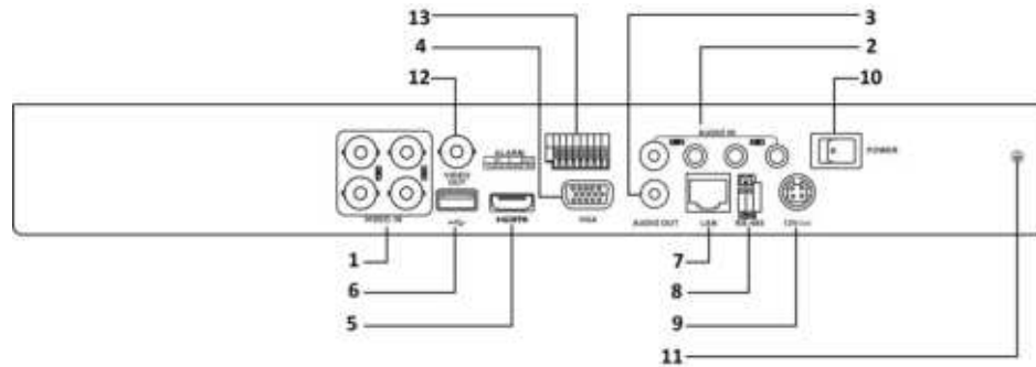
Figure 1. 4 Rear Panel
