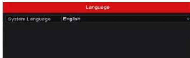
Figure 2. 6 Language Configuration
