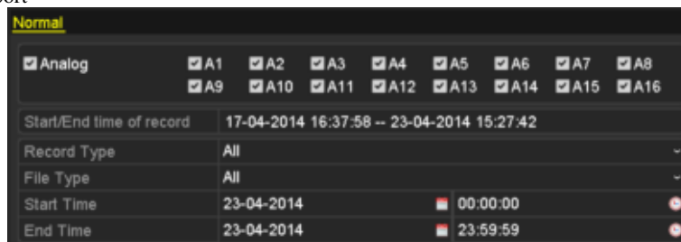
Figure 5.29 Export
