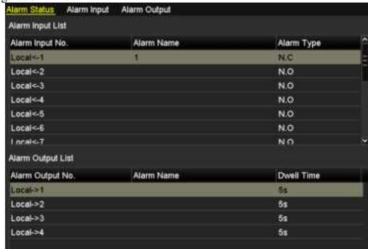
Figure 5.15 Alarm Settings
