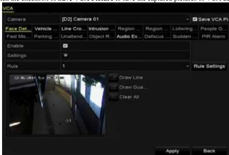
Figure 9. 1 Face Detection
