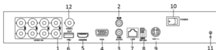
Figure 1. 5 Rear Panel 1
