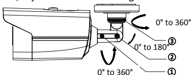
Figure 2-10 3-Axis Adjustment
