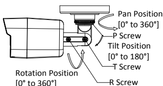
Figure 2-3 3-axis Adjustment
