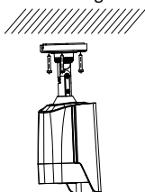
Figure 2-9 Fix the Camera to the Ceiling
