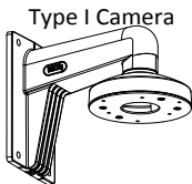
Figure 2-17 Install the Bracket
