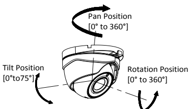
Figure 2-14 3-axis Adjustment
