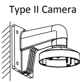
Figure 2-17 Install the Bracket
