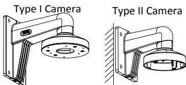
Figure 2-17 Install the Bracket
