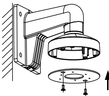
Figure 2-14 Install the Adapter to the Pendent Cap
