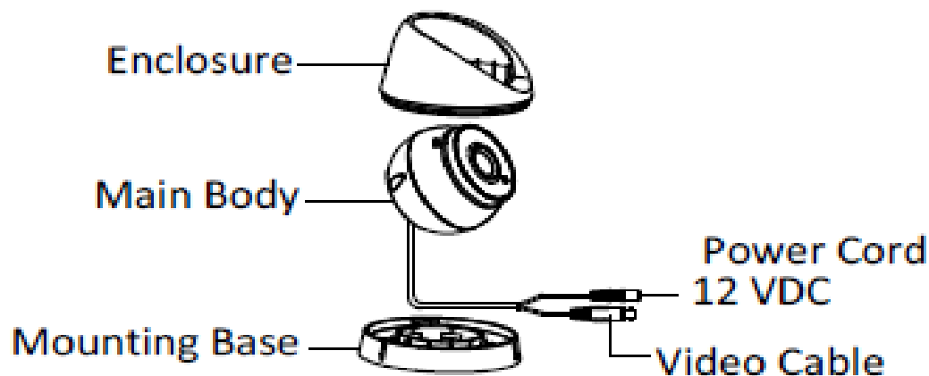
Figure 1-1 Overview of Type I Camera
