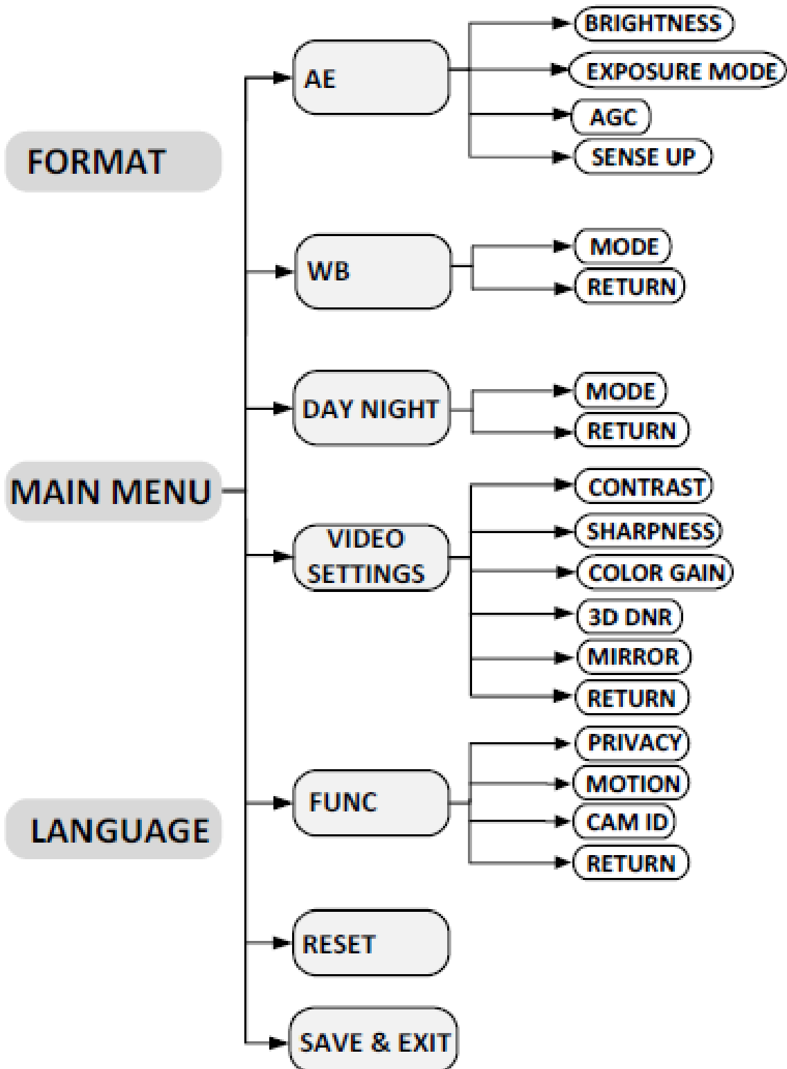
Figure 3-2 Main Menu Overview
