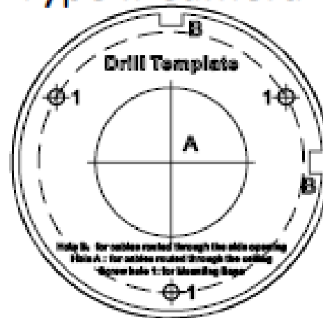
Figure 2-15 Drill Template of the Junction Box
