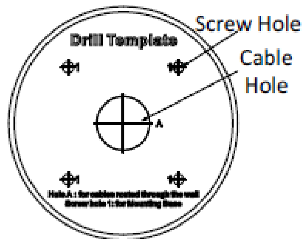
Figure 2-6 The Drill Template
