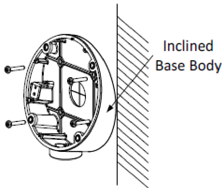
Figure 2-8 Fix the Inclined Base Body
