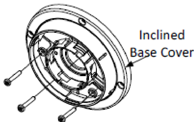
Figure 2-7 Install Turret Camera's Mounting Base
