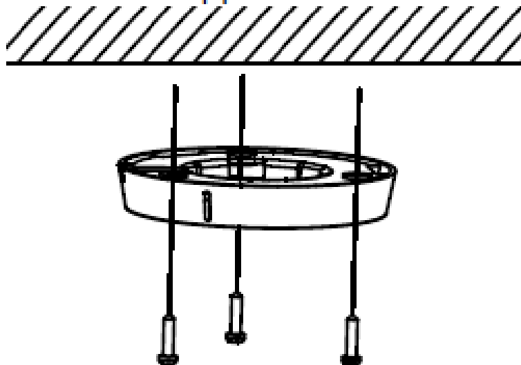
Figure 2-3 Attach the Mounting Base to the Ceiling
