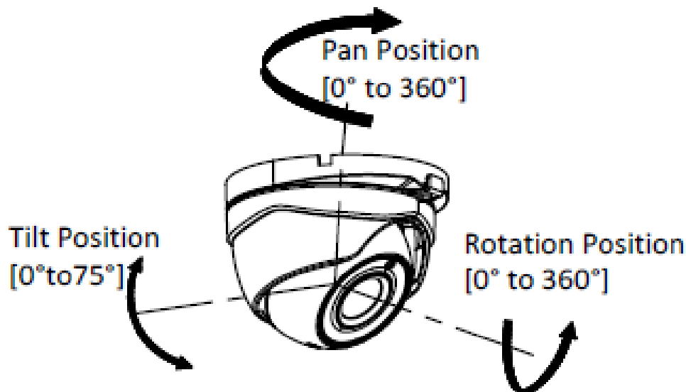
Figure 2-14 3-axis Adjustment
