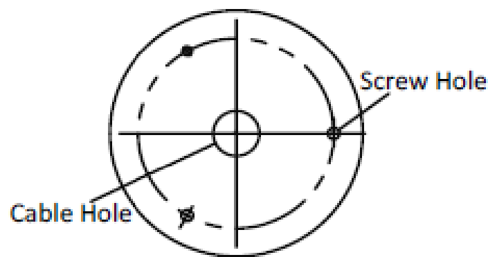
Figure 2-2 Drill Template
