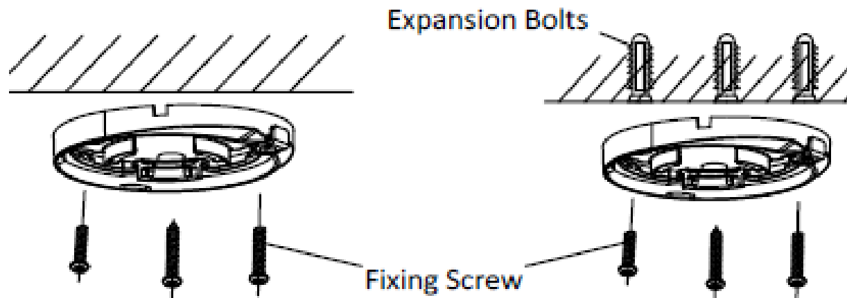
Figure 2-12 Fix the Mounting Base to the Ceiling
