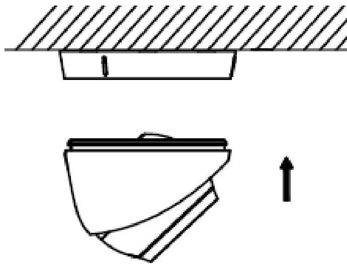
Figure 2-4 Secure the Camera with Mounting Base
