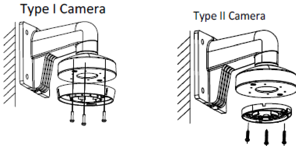
Figure 2-18 Install the Mounting Base to the Bracket
