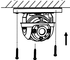
Figure 2-3 Fix the Mounting Base and Camera
