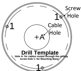
Figure 2-19 Drill Template
