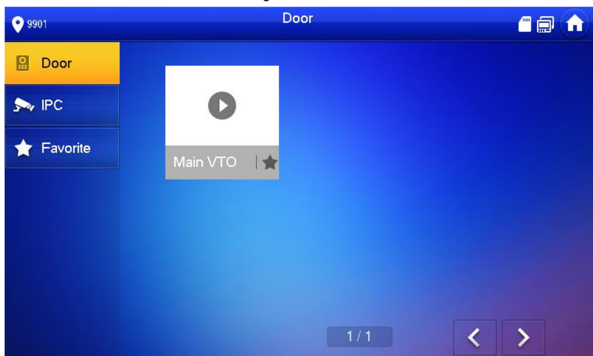
Figure 2-16 Door
