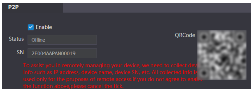
Figure 3-4 P2P
