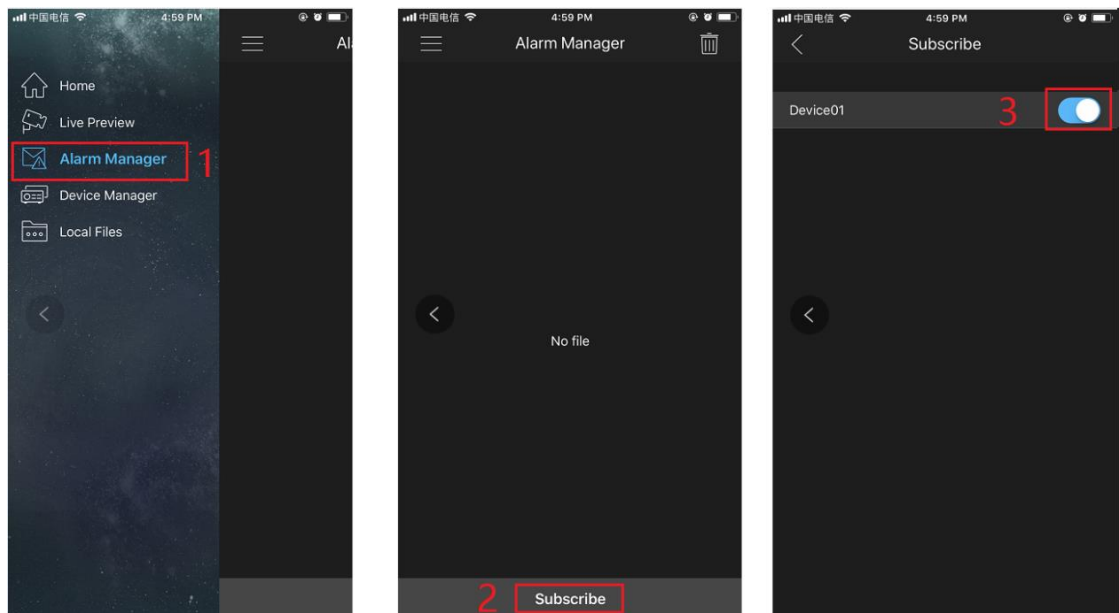
Figure 3-6 Subscribe
