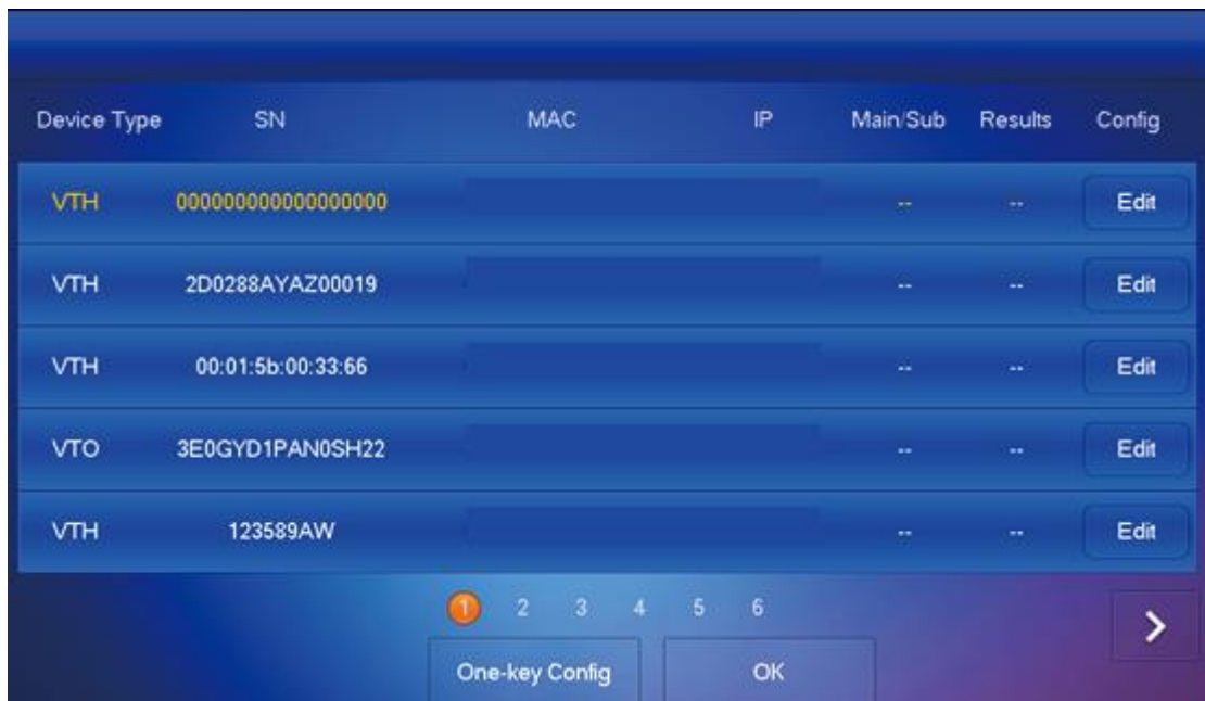
Figure 2-11 Configuration interface
