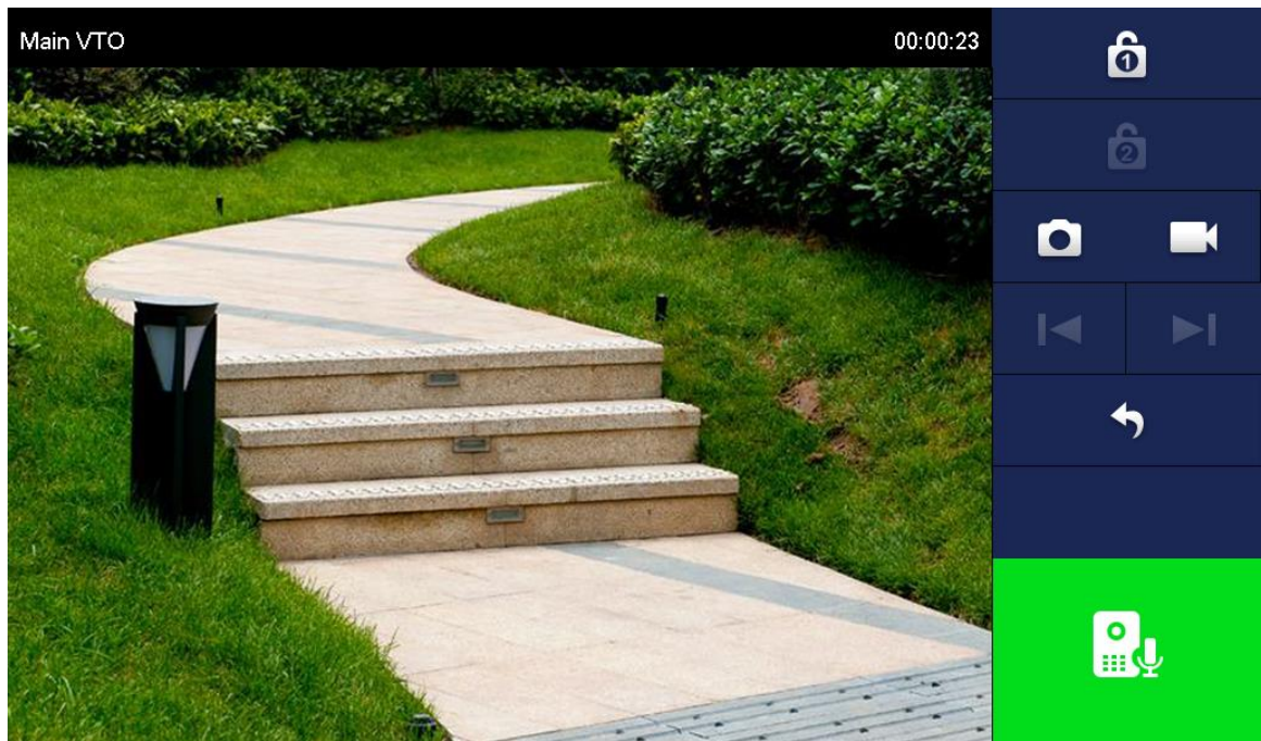
Figure 2-17 Monitoring video
