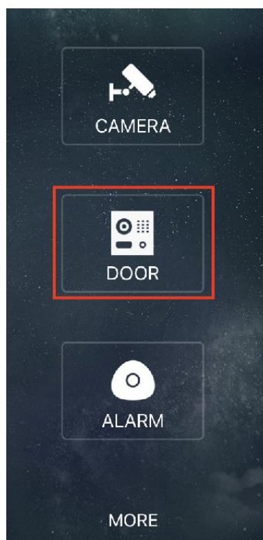
Figure 3-2 Home page
