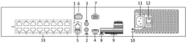
Rear Panel of NVR-PRE32C-16P4K
