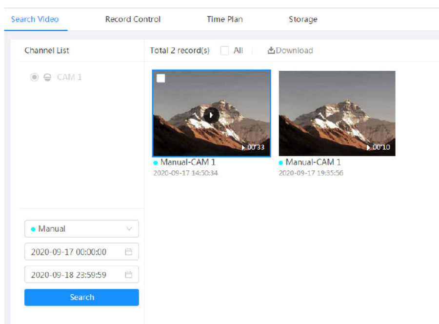
Figure 7-1 Search video
