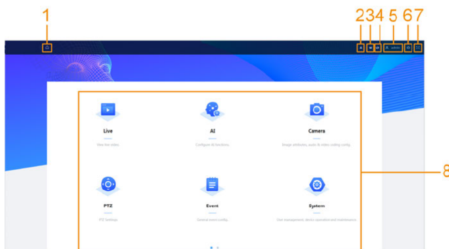
Figure 4-2 Main page
