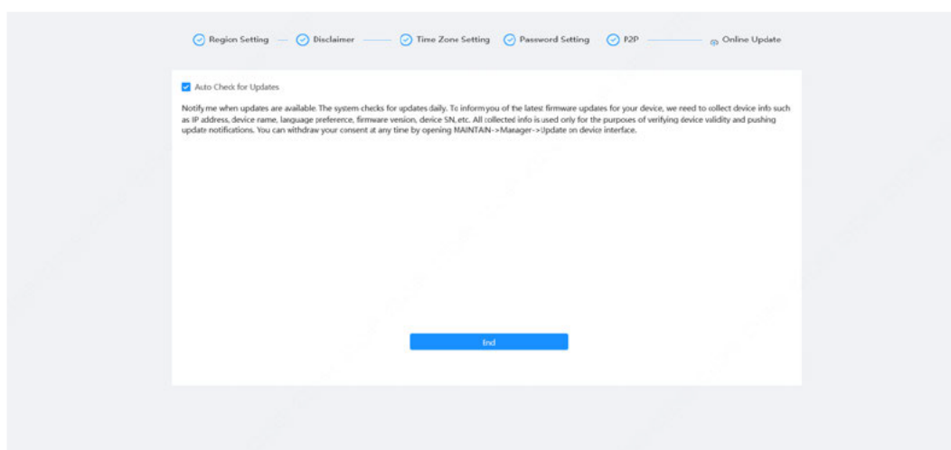
Figure 3-6 Online update
