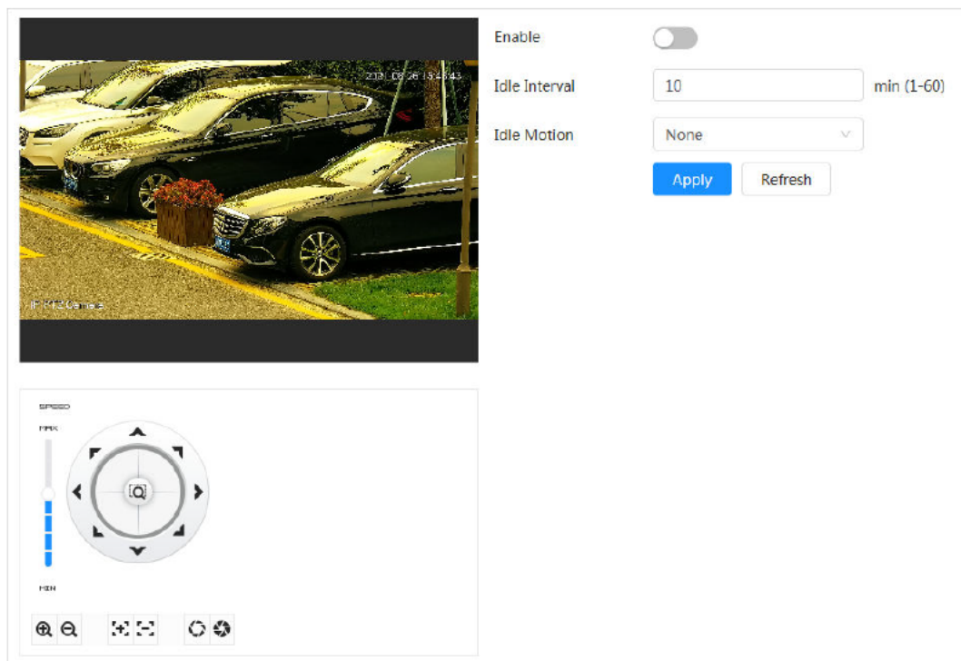
Figure 4-59 Idle motion
