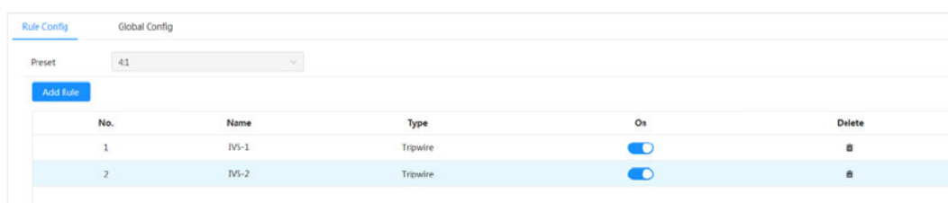
Figure 9-21 Tripwire
