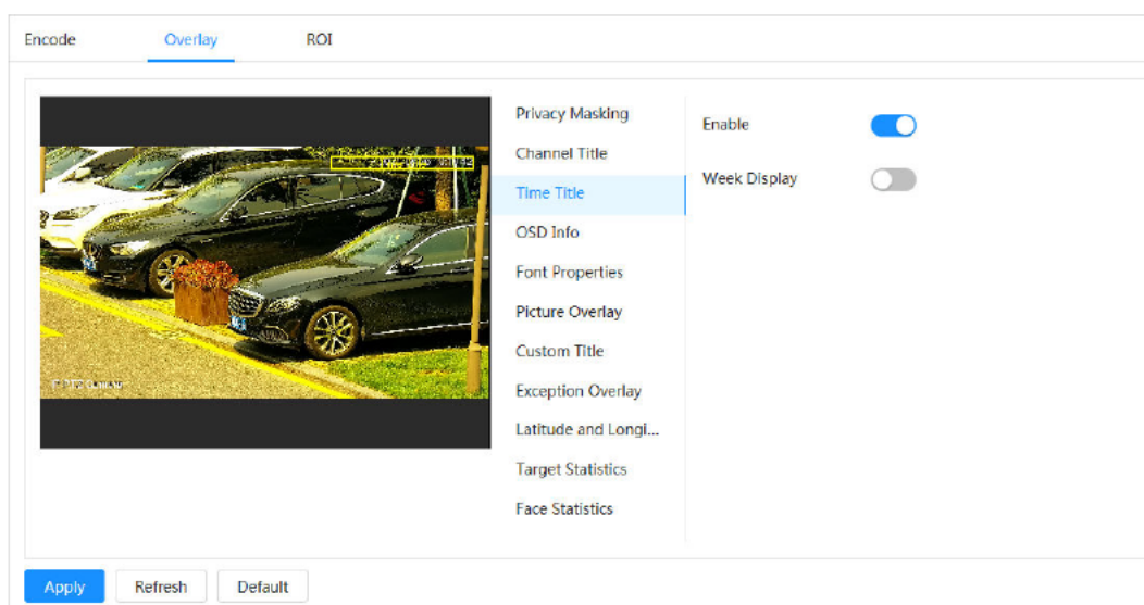
Figure 4-20 Time title
