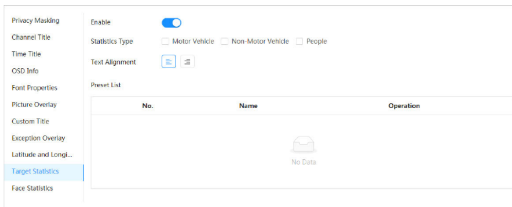
Figure 4-27 Target statistics
